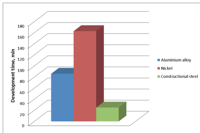
Fig.12. Average development times for tested materials
