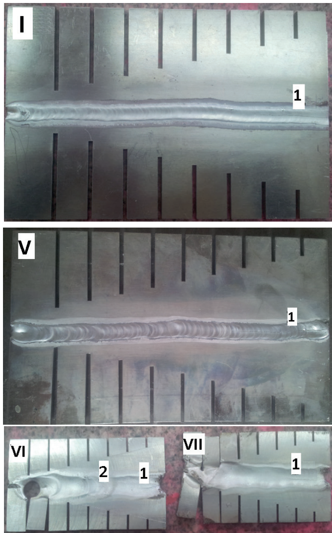
Fig. 3. Sheets with notches in similarity to the Houldcraft’s test after TIG penetration (visible cracks). Roman numerals indicate the serial number of the joint while Arabian ones indicate the serial number of the crack in the joint
