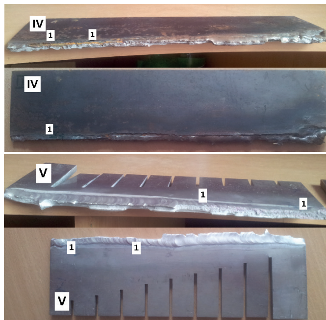
Fig. 13. Selected butt joints after breaking in the place of cracks. In the upper portion of the photo the part of butt joint in constructional steel is visible; in the lower – that of aluminium alloy. The Roman numerals indicate the serial number of the joint while the Arabian ones – the serial number of the crack in the joint
