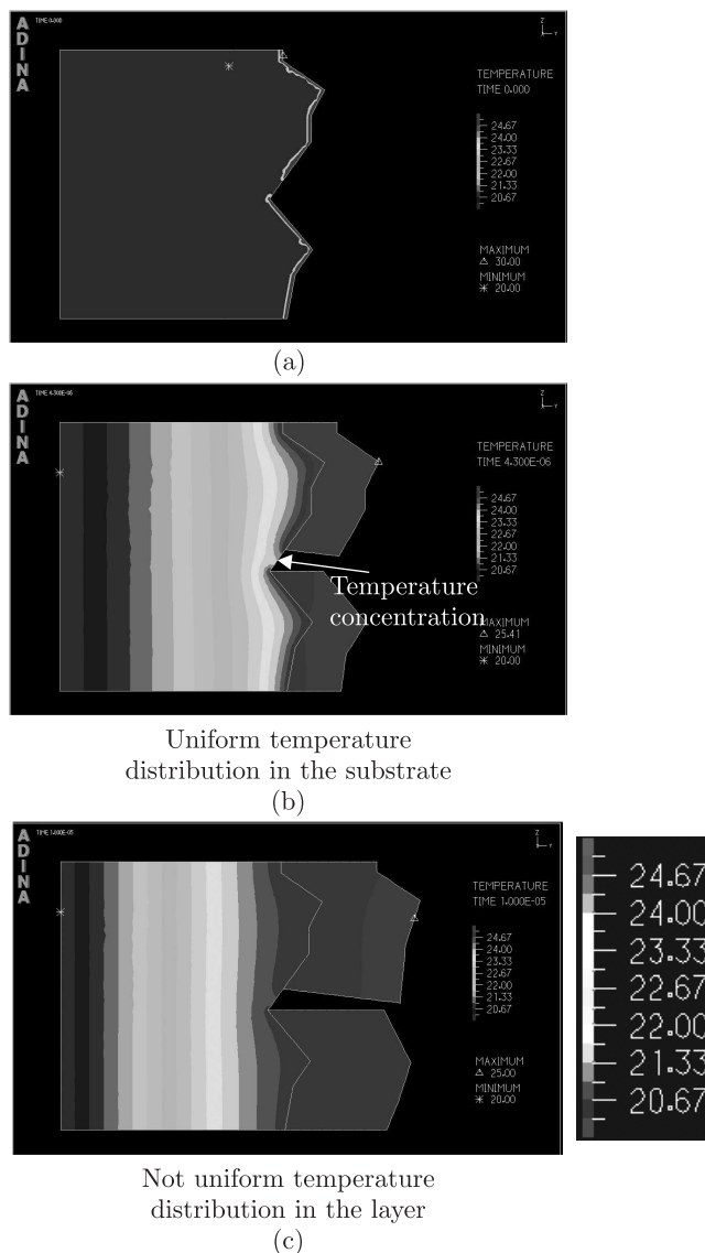
Fig. 13. Temperature distribution in the composition during deposition process; (a) initial stage, (b) medium stage, (c) late stage
