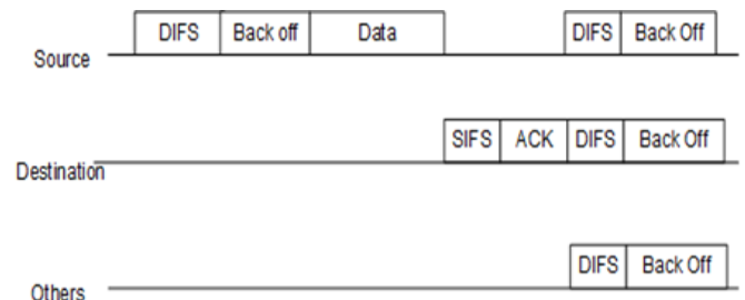
Fig. 3. Basic access mechanism in IEEE802.11 dcf mac
