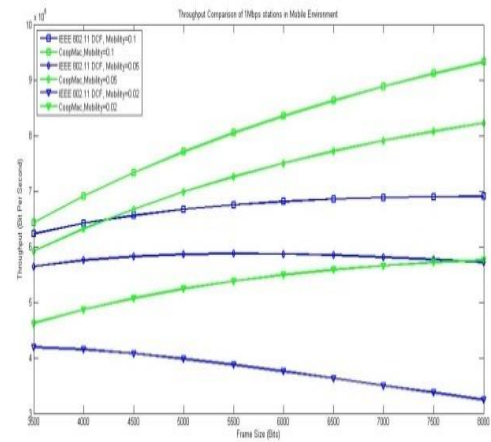
Fig.13.Throughput comparison of 1 Mbps stations with mobility
