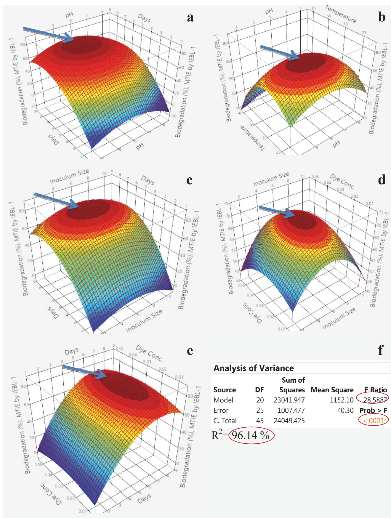
Fig. 1. Response surface 3D graphs showing interaction between various parameters during the biodegradation of Mujahid Textile (MT) industrial effluent by Coniophora puteana IEBL-1, graphs represent positive interaction between (a) time period and pH (b) temperature and pH (c) time period and inoculum size (d) dye concentration and inoculum size (e) dye concentration and time period (f) statistical analysis of results showing significant effect of parameters on biodegradation
