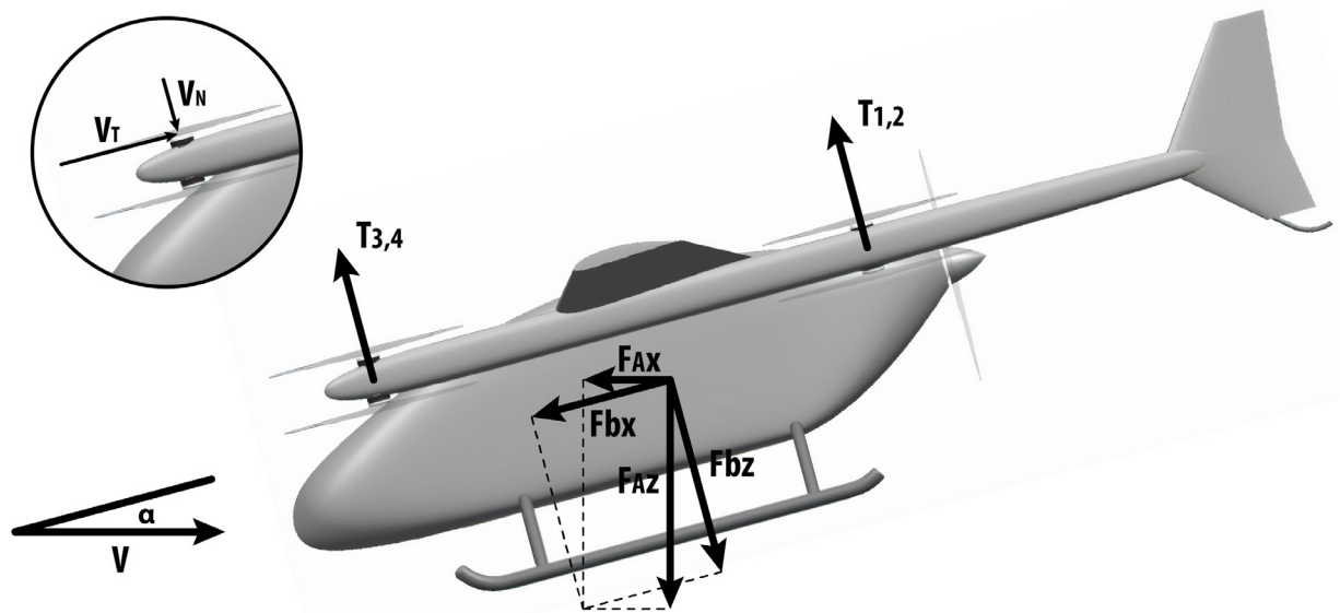
Fig. 10. Propulsion forces at an angle of attack
