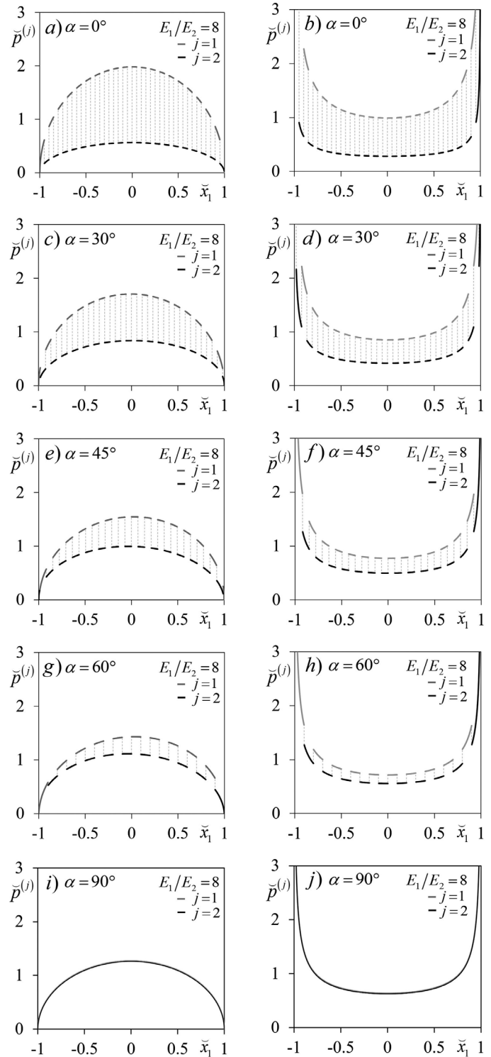
Fig. 2. Contact pressures \check{p}^{(j)}(\check{x}_1) = p^{(j)}(\check{x}_1) / p_0 , j = 1, 2 for j -th component of the composite body at E_1/E_2 = 8 , \nu_1 = \nu_2 = 0.3 , \eta = 0.5 for different lamina angles and different punch shapes: a), c), e), g), i) – parabolic punch, b), d), f), h), j) – rectangular punch
