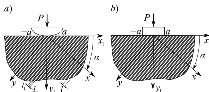
Fig. 1. Scheme of considered contact problems for: a) parabolic punch, b) rectangular punch
