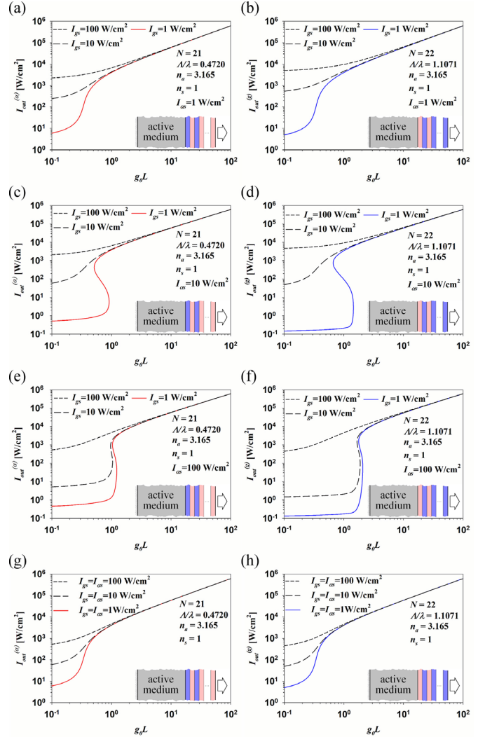
Fig. 7. Output intensity I_{\text{out}}^{(\{\alpha,g\})} of the laser in discrete configuration, plotted as a function of normalized small-signal gain coefficient g_0 L for various loss I_{s\alpha} and gain I_{sg} saturation intensities of the mirror loss and gain layers: (a) and (b) I_{s\alpha} = 1 \text{ W/cm}^2 and I_{sg} = 1, 10, 100 \text{ W/cm}^2 ; (c) and (d) I_{s\alpha} = 10 \text{ W/cm}^2 and I_{sg} = 1, 10, 100 \text{ W/cm}^2 ; (e) and (f) I_{s\alpha} = 100 \text{ W/cm}^2 and I_{sg} = 1, 10, 100 \text{ W/cm}^2 ; (g) and (h) I_{sg} = I_{s\alpha} = 1, 10, 100 \text{ W/cm}^2 . Characteristics in the left column – for setup 1, right column – setup 2
