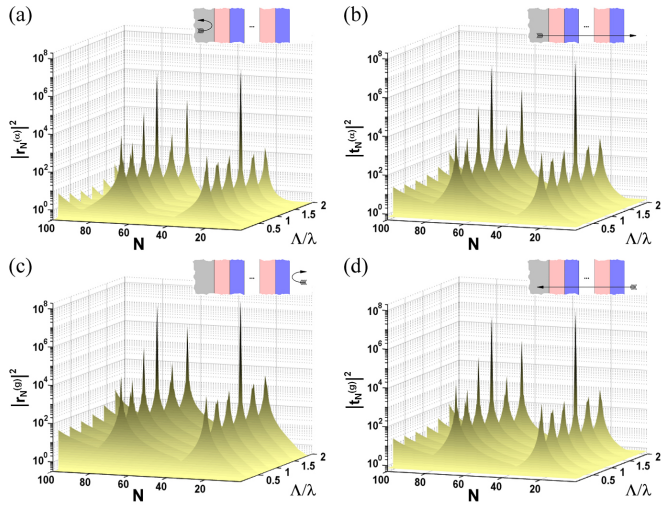
Fig. 4. Reflection |r_N^{(\alpha,g)}|^2 and transmission |t_N^{(\alpha,g)}|^2 coefficients of a linear PT mirror in discrete configuration for setup 2. These coefficients are plotted as a function of the number N of primitive cells and the ratio \Lambda/\lambda . In (a) and (b), the electromagnetic waves incident on the gain layer. In (c) and (d), the electromagnetic wave is incident on the loss layer
