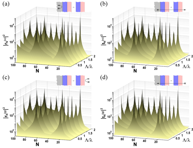
Fig. 3. Reflection |r_N^{(\alpha,g)}|^2 and transmission |t_N^{(\alpha,g)}|^2 coefficients of a linear PT mirror in discrete configuration for setup 1. These coefficients are plotted as a function of the number N of primitive cells and the ratio \Lambda/\lambda . In (a) and (b), the electromagnetic wave is incident on the loss layer. In (c) and (d), the electromagnetic wave is incident on the gain layer
