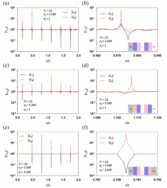
Fig. 6. Eigenvalues \lambda_1 , \lambda_2 shown as a function of ratio \Lambda/\lambda for PT mirror structures. Figures on the right side show more precisely the behavior of the eigenvalue highest maxima observed in the corresponding figures presented on the left side. Figures (a)–(d) characteristics are plotted for a PT mirror in discrete configuration (a) and (b) for setup 1 and parameters highlighted in Table 1; (c) and (d) for setup 2 and parameters highlighted in Table 2. Figures (e) and (f) show characteristics for the PT mirror in integrated configuration of a laser for parameters highlighted in Table 3
