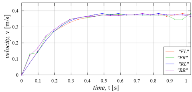
Fig. 7. The velocity course of the set pulses of the drive torques of the wheels in the first phase of the movement
