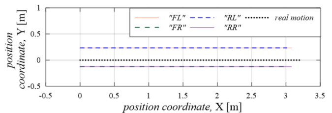
Fig. 9. Movement trajectory with the track of road wheels and a selected point of the robot's body in real motion
