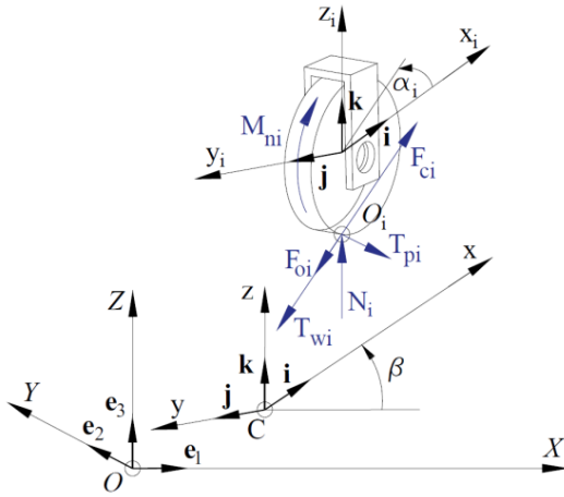
Fig. 2. Forces in the frame of reference during motion
