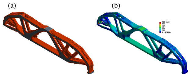
Fig. 14. The SIMP algorithm: the validated solution (a), the contour map of Huber–Mises–Hencky's equivalent stress [MPa] (b)
