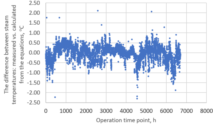
Figure 6: The difference between steam temperatures: measured vs. calculated from Eqs. (15) and (16).
