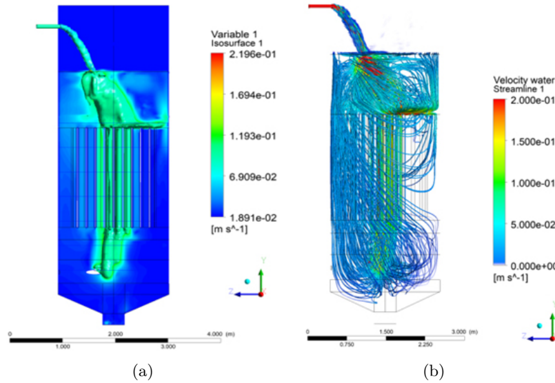
Figure 3: Numerical evaluation of the flow in the fermentor: a) velocity isosurface – quality view of the main mixing area and where the highest velocities occur; b) streamlines – view of the recirculation zone.
