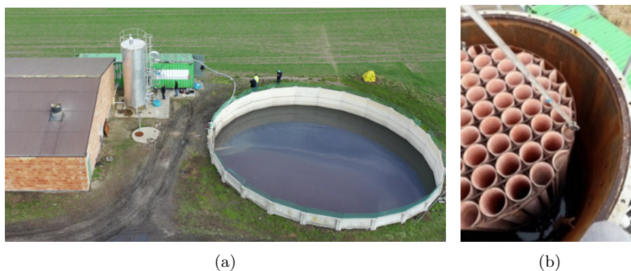
Figure 1: Pilot biogas plant: (a) location of the biogas plant – from the right: a fragment of a piggery building, a monosubstrate flow reactor for meta-new liquid manure fermentation with an installation for the production of agricultural biogas, a lagoon for post-fermentation; (b) an adhesive bed made of vertical pipes with a roughness of 80 \mu\text{m} , transported to the inside of the fermenter.
