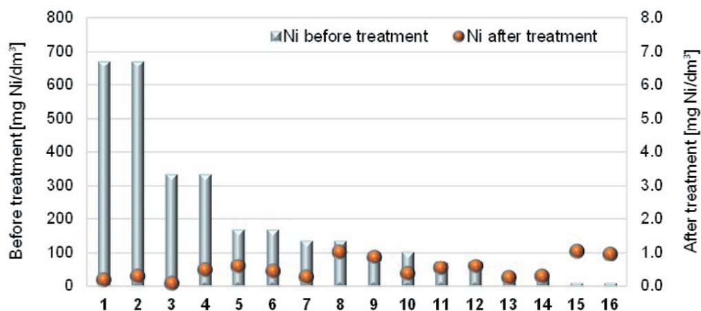
Fig. 3. Nickel content in the model PIWW before and after neutralization for different initial concentrations
