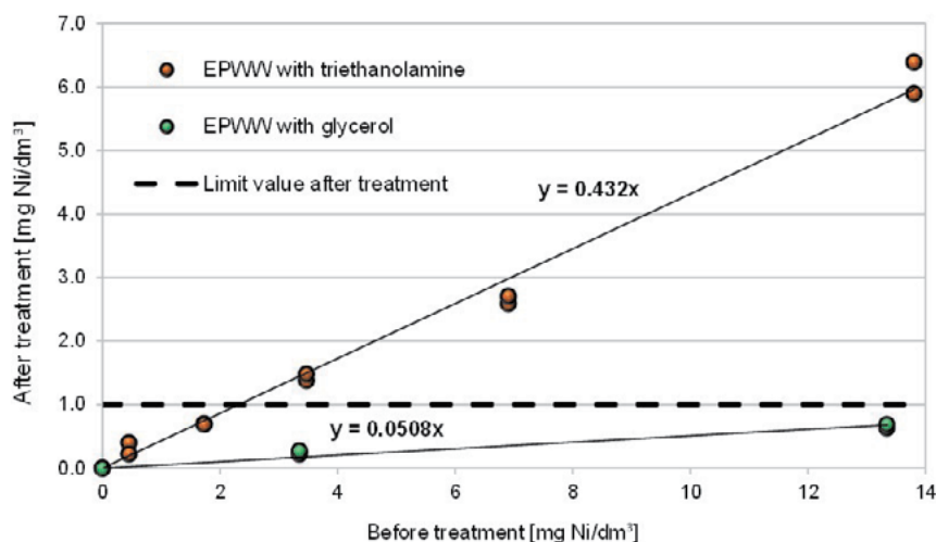
Fig. 4. Nickel content before and after neutralization for the model EPWW with both either triethanolamine or glycerol
