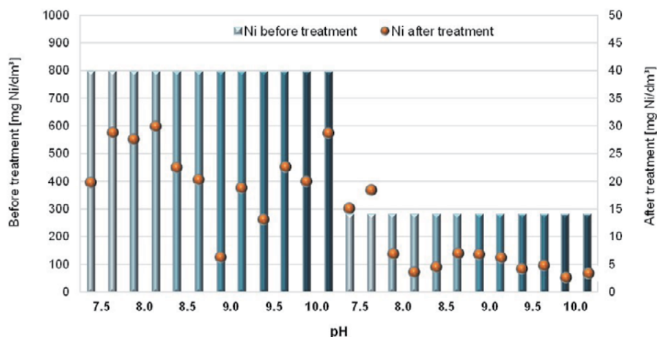
Fig. 5. Nickel content in the PIWW + EPWW before and after neutralization for different initial concentrations
