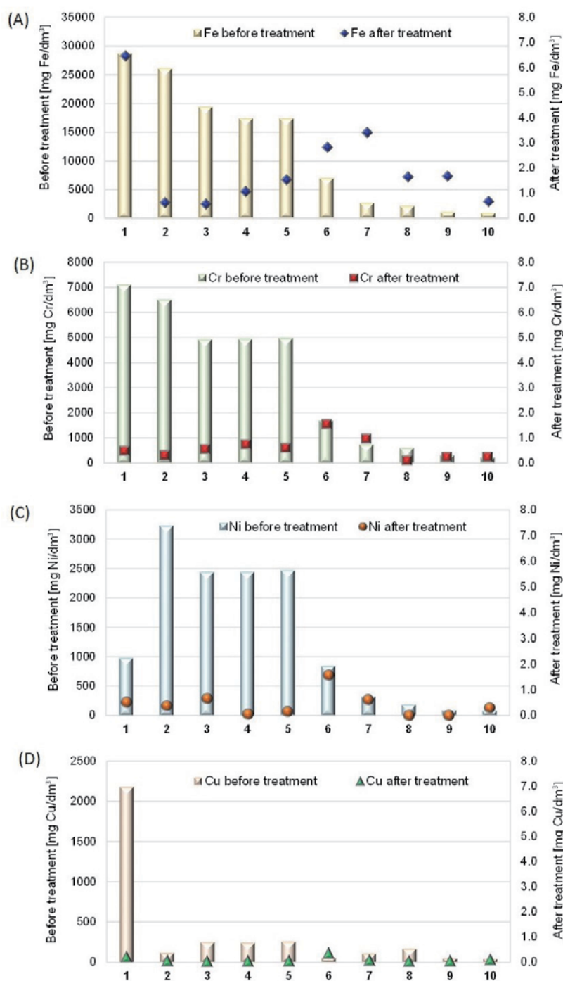
Fig. 6. Comparison of iron (A), chromium (B), nickel (C), copper (D) ions in industrial wastewater from pickling and electropolishing for a series of 10 technical tests before and after neutralization
