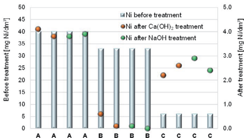
Fig. 2. The content of nickel ions before and after the neutralization process with the use of either calcium hydroxide or sodium hydroxide for model wastewater: A) PIWW + EPWW, B) PIWW, C) EPWW.
