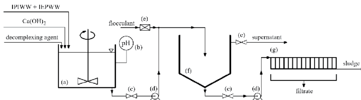
Fig. 1. Simplified diagram of the installation for treatment and neutralization of wastewater from steel pickling and electropolishing processes a) neutralization chamber, b) pH-meter, c) valve, d) pump, e) non-return valve, f) settling tank, g) filter press
