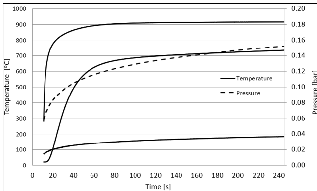
Fig. 3. Simulated temperature and pressure changes
