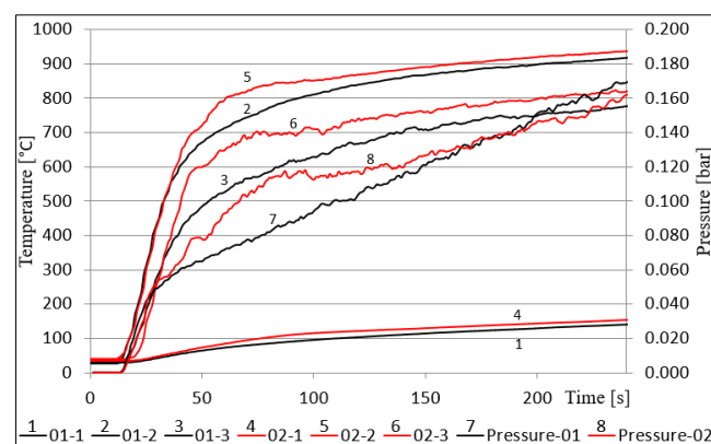
Fig. 7. Summary of temperature and pressure results as a function of time. 4, 5, 6, 8 - heating process with polystyrene sample. 1, 2, 3, 7 - heating process without polystyrene sample
