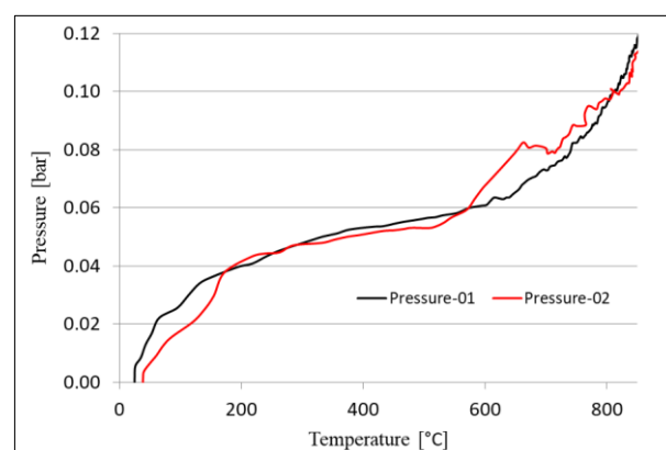
Fig. 9. Dependency graph pressure - temperature - sample number 5
