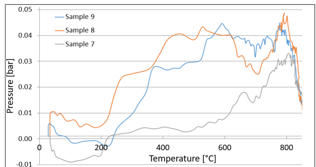
Fig. 15. Pressure difference as a function of temperature for samples 7-9
