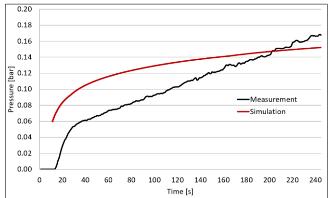
Fig. 6. Pressure changes curves in the combustion chamber, simulation, and measurement results during tests
