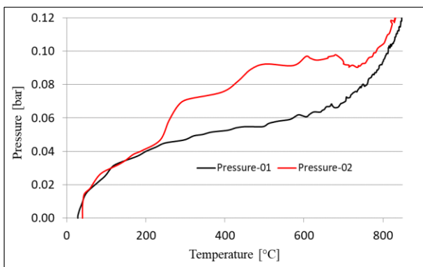
Fig. 12. Dependency graph pressure - temperature -sample number 8
