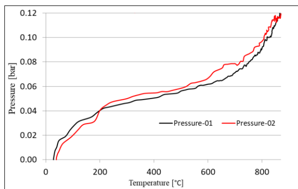
Fig. 10. Dependency graph pressure - temperature - sample number 6
