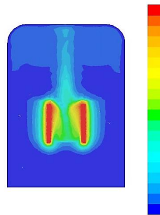
Fig. 2. Temperature field in the measuring chamber – simulation results
