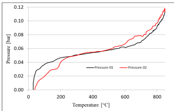
Fig. 11. Dependency graph pressure - temperature -sample number 7
