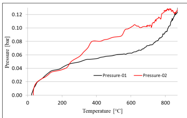
Fig. 13. Dependency graph pressure - temperature - sample number 9
