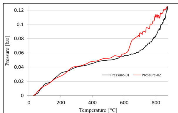
Fig. 8. Dependency graph pressure - temperature - sample number 4
