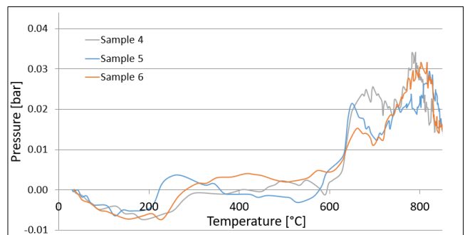
Fig. 14. Pressure difference as a function of temperature for samples 4-6
