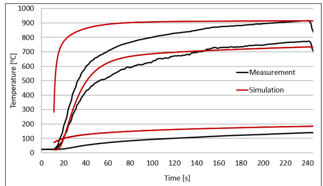
Fig. 5. Temperature change curves in the combustion chamber, simulation, and measurement results during tests
