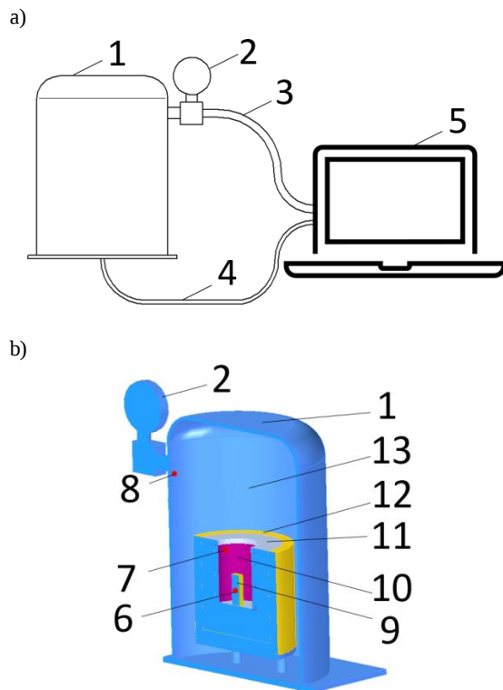
Fig. 1. Measuring stand. a) workstation's schematics; b) view in the section of the combustion chamber.
