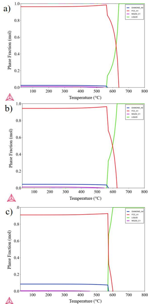
Fig. 2. Temperature-dependent phase fraction graphs of alloys a) AlSi5 b) AlSi7 c) AlSi9
