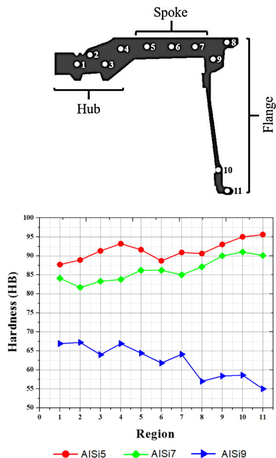
Fig. 12. Hardness values for AlSi5, AlSi7 and AlSi9 alloys and measurement points on the wheel section
