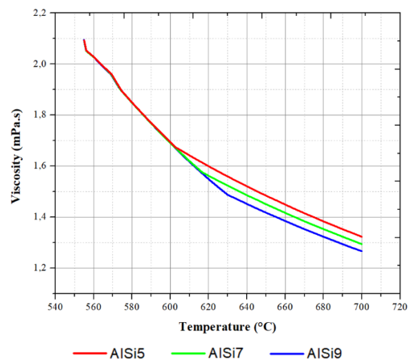
Fig. 4. Viscosity-temperature graphs for studied alloys
