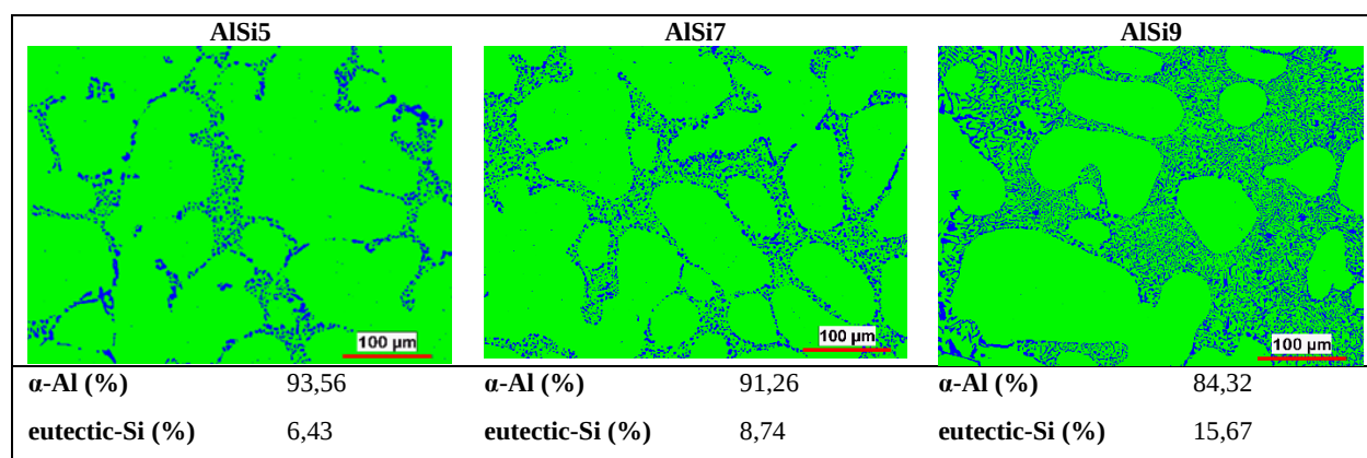
Fig. 7. Phase amount calculations for studied alloys
