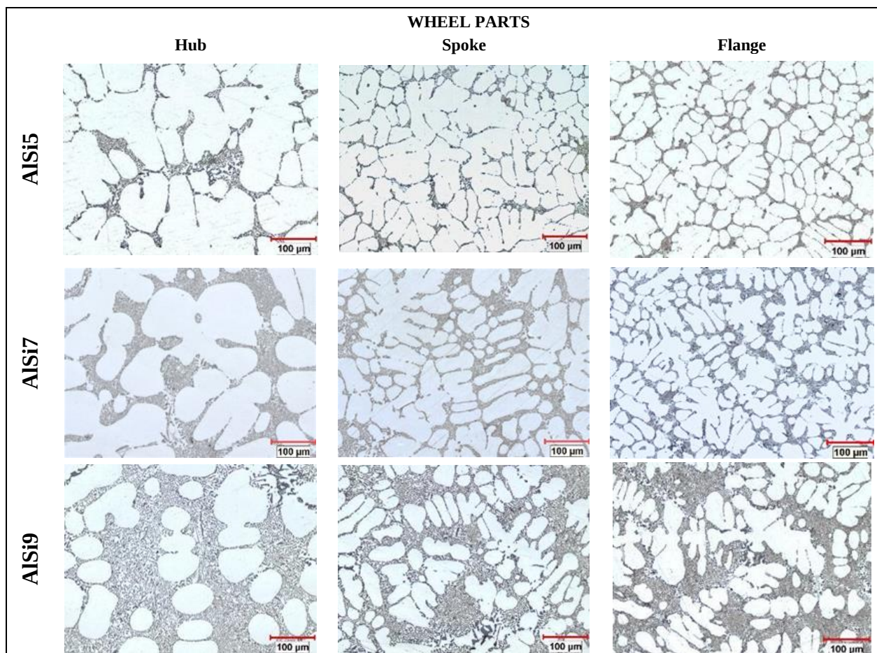
Fig. 6. Optical microscope images of the AlSi5, AlSi7 and AlSi9 alloys
