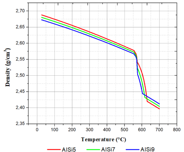
Fig. 5. Temperature-dependent density values graphs for studied alloys
