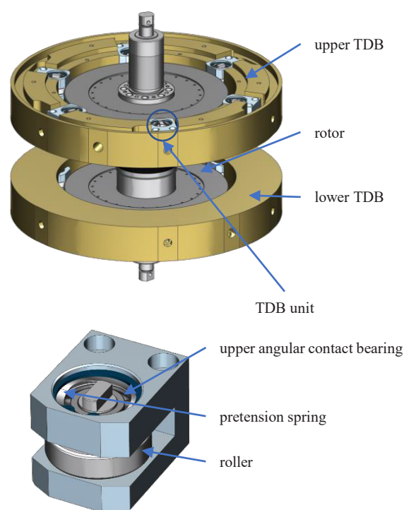
Fig. 1. Rotor of the TDB test rig with planetary TDB in the stator and a single TDB unit
