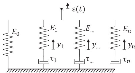
Fig. 4. Model for the dynamic stiffness of elastomers
