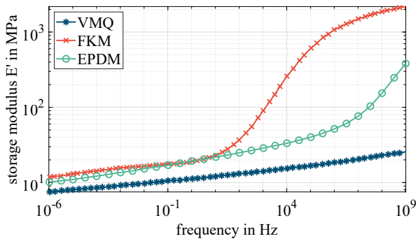
Fig. 2. Storage modulus of investigated materials [7]
