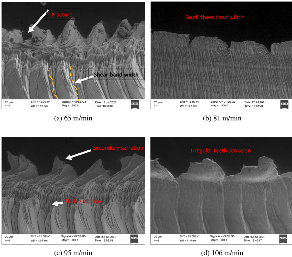
Fig. 3. Chip obtained during the increase in various cutting speeds for machining Inconel 718
