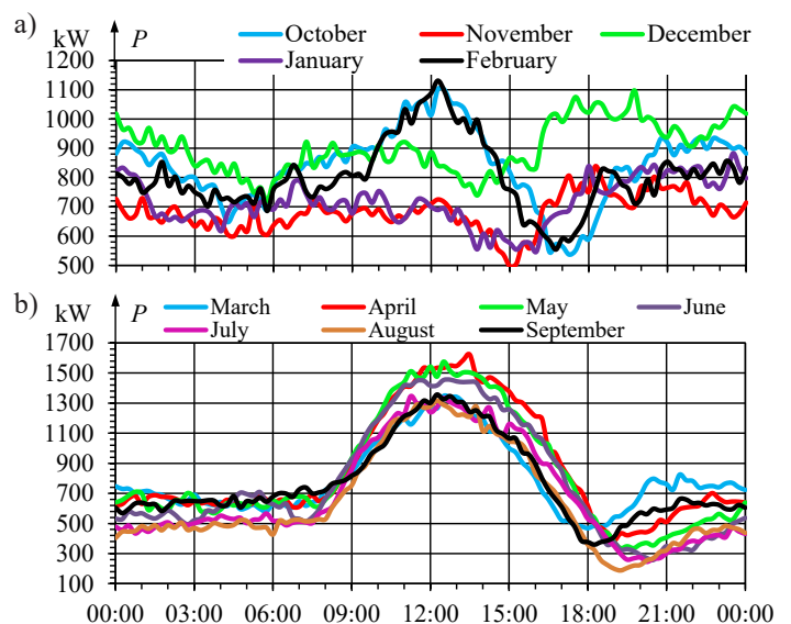
Fig. 33. Median of 6 years of active power generated by a 2 MW photovoltaic power plant and a 2 MW wind power plant in individual day quarters to the power grid, broken down into months
