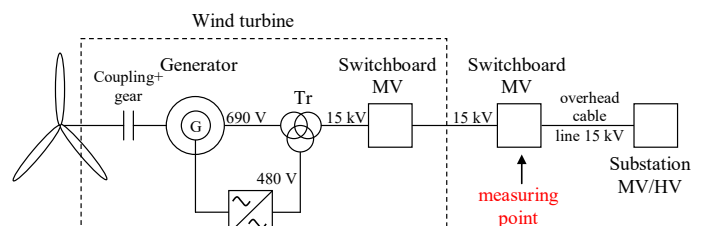
Fig. 2. Simplified diagram of the wind power station [50]
