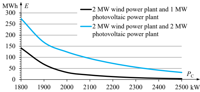
Fig. 28. The 6-year average of energy not generated to the power grid in a year due to connection capacity PC constraints depending on the value of connection capacity for the combined 2 MW wind power plant and 1 MW photovoltaic power plant and the combined 2 MW wind power plant and 2 MW photovoltaic power plant
