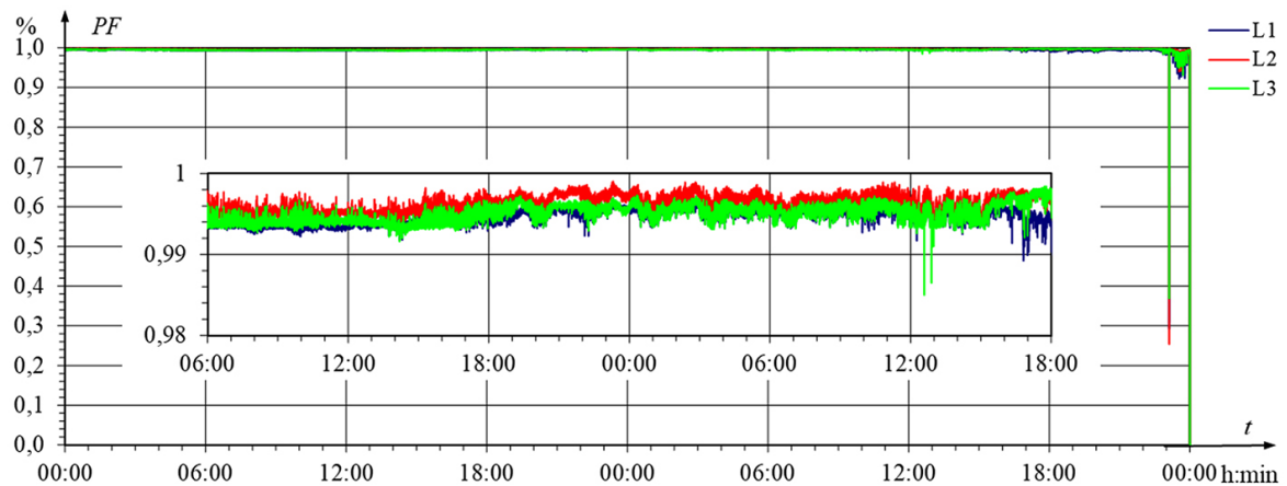
Fig. 18. Variations of the power factor of the load drawn by the wind power plant
