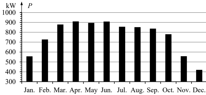
Fig. 3. The maximum active power (15 min. interval) generated by the PV power station in individual months (six-year maximum values)
