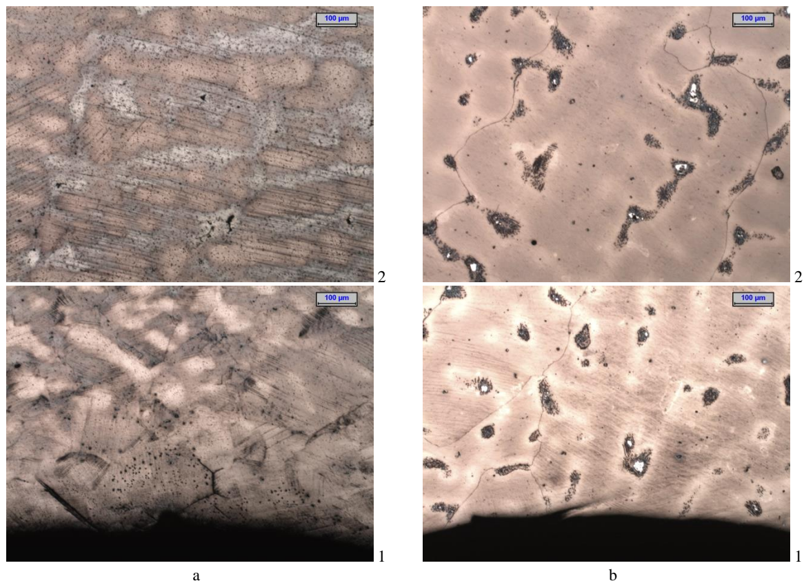
Fig. 8. Cast steel microstructure in the area of load impact from three zones; 100x; light microscope, nital etching
