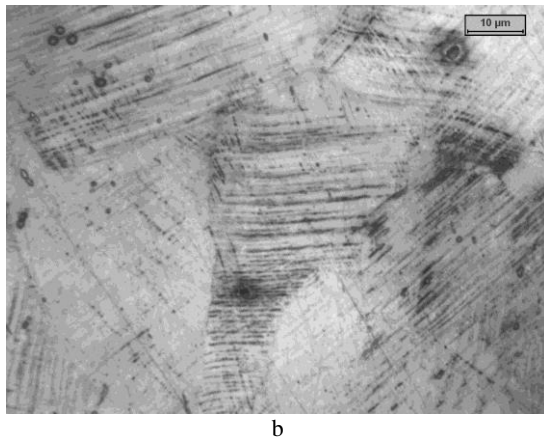
Fig. 9. The microstructure of GX120Mn13 cast steel in zone 2; light microscope, nital etching
