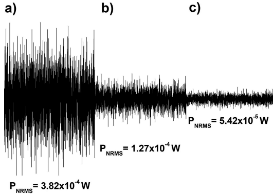
Fig. 5. Laser radiation intensity noise measured by the PSD. The optical power of the beam was 3 mW for every aperture slit. The sections in the graph correspond with a) standard laser configuration with APC control, b) laser with APC and RF modulated bias current, c) laser with APC and an RF modulated bias current and a 0.8 mm slit aperture in the optical path.
