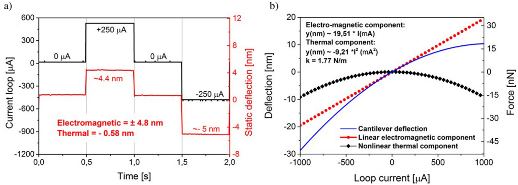
Fig. 10. a) Cantilever static deflection in response to a step function signal; b) Pseudo-static (low frequency) actuation characteristics of a 1.77 N/m microcantilever measured in 0.48 T magnetic field with thermal and magnetic actuation components extracted.
