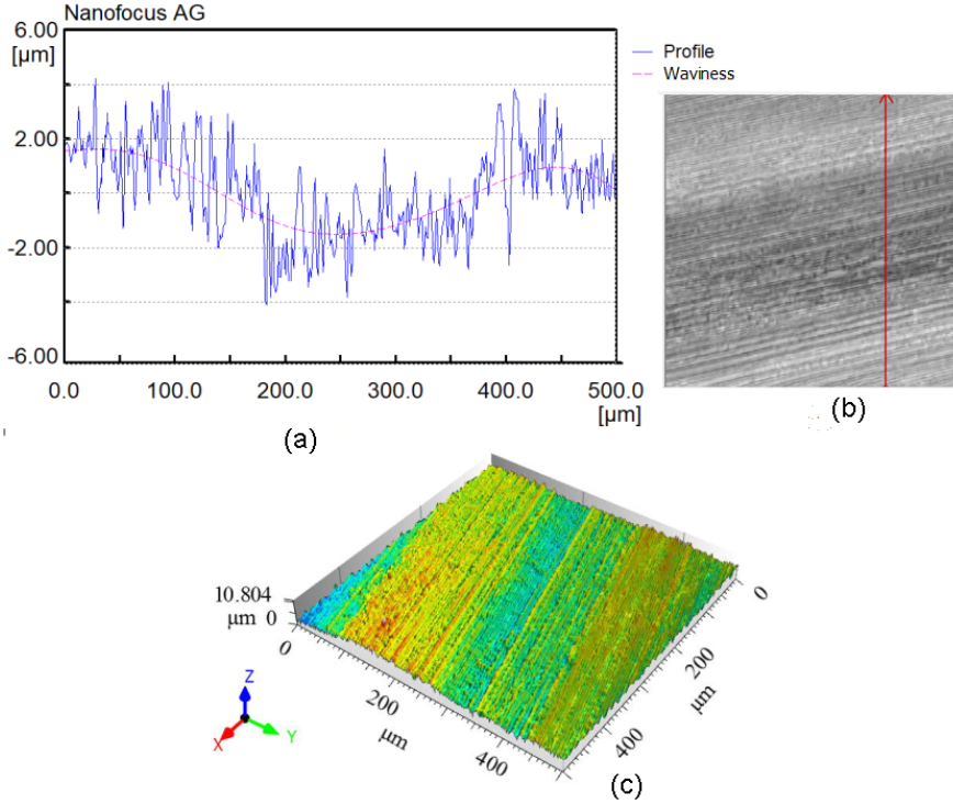
Fig. 3. Example of profile waviness and roughness for the test piece made of steel 100Cr6: (a) a_p = 0.2 mm, f = 0.25 mm/rev, v = 817 mm/min, 62 HRC, SW_t = 3.067 µm, Ra = 0.937 µm; cut-off \lambda_c = 0.8 mm;), recorded with the \mu scan laser profilometer by Nano focus and the Nanofocus AG software; (b) – position of the sectioning plan for obtaining the image in figure (c); (c) – profile analyzed with the optical 3D measuring system for the same test piece, elaborated by means of the 3D optical noncontact measuring system produced by MahrFederal.
