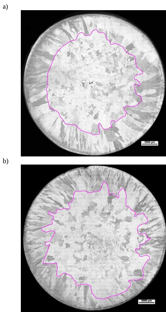
Fig. 3. Macrostructure of examined steel, (a) in initial state, (b) after SiZr inoculation
