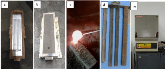
Fig. 2. The steps of the sand casting method
