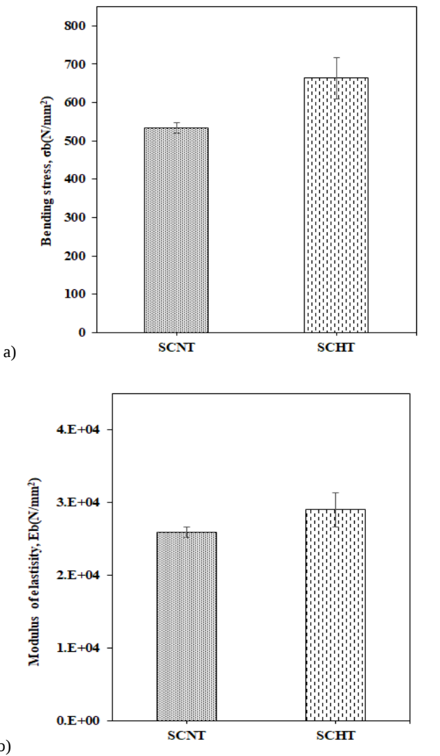
Fig. 9. (a) The bending strength Cu20wt.%Sn (b) The modulus of elasticity Cu20wt.%Sn
