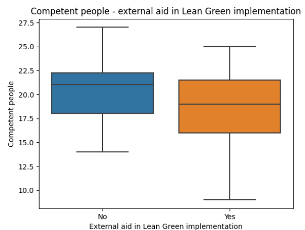
Fig. 13. Boxplot – Competent people by external aid in Lean Green implementation
