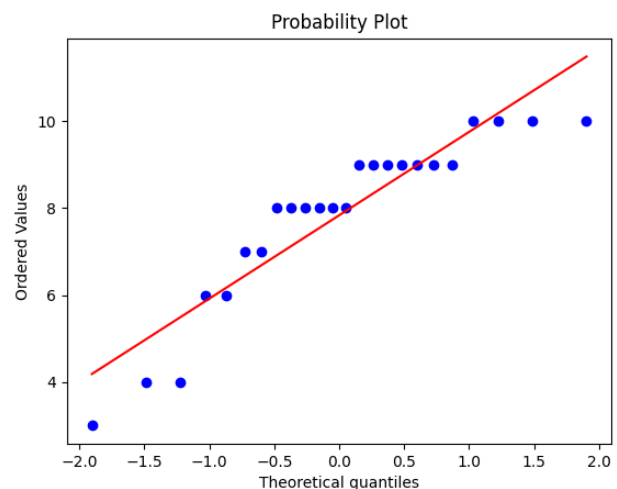
Fig. 17. Probability Plot – Correctly functioning communication system by external aid in Lean Green implementation
