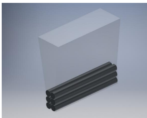
Fig. 5. YII shape casting with specimens for metallographic and mechanical properties examinations
