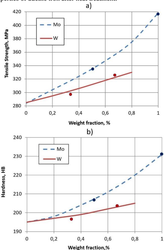
Fig. 3. The influence of molybdenum and tungsten on the tensile strength and HB hardness of grey cast iron [4]
