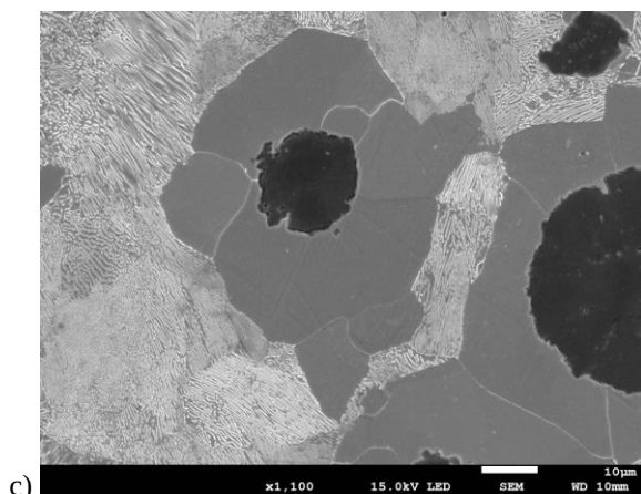
Fig. 6. Microstructure of DI-Cu ductile iron
