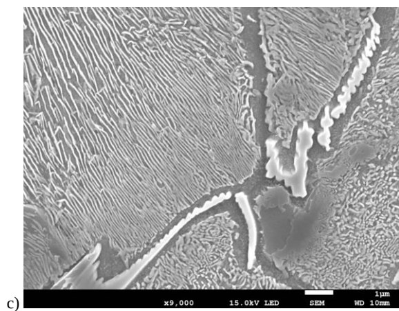
Fig. 8. Microstructure of DI-CuW2 ductile iron
