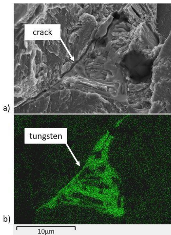
Fig. 10. Brittle fracture at the carbide-matrix interface in DI-CuW3 cast iron; a) SEM photo, b) indication of the presence of tungsten on EDS mapping
