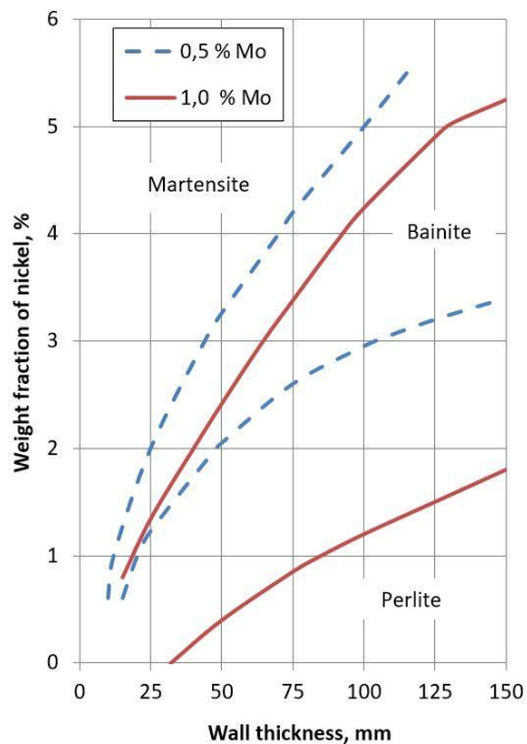
Fig. 2. Structural diagram of low-alloy gray cast iron containing Ni and Mo depending on the wall thickness; continuous line - 1.0% Mo; dashed line - 0.5% Mo [4]
