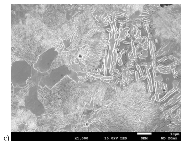
Fig. 9. Microstructure of DI-CuW3 ductile iron
