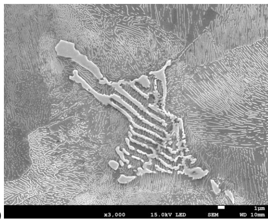
Fig. 7. Microstructure of DI-CuW1 ductile iron
