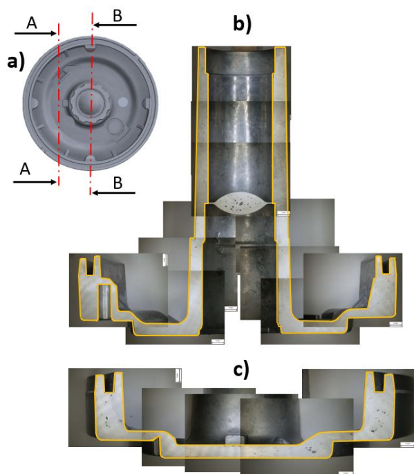
Fig. 2. Example of control sections by casting A55; a) Location of sections; b) Section B-B castings; c) Section A-A castings
