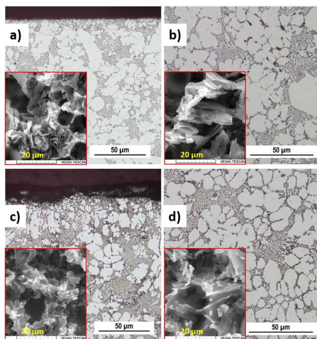
Fig. 4. Microstructure of casting A10 and A55 (OM – etc. Dix-Keller, SEM – etch. HCl); (a) surface area A10; (b) central region A10; (c) surface area A55; (d) central region A55
