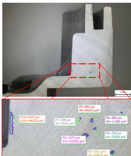
Fig. 3. Methodology of measuring areal porosity on control sections
