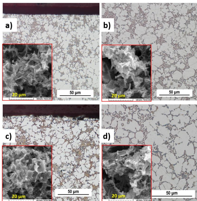
Fig. 5. Microstructure of casting A75 and A90 (OM – etc. Dix-Keller, SEM – etch. HCl); (a) surface area A75; (b) central region A75; c) surface area A90; (d) central region A90
