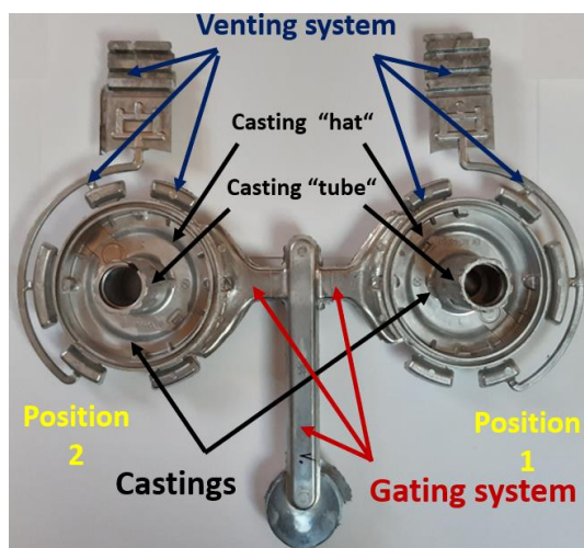
Fig. 1. The geometry of casting Buchse in double cavity mould
