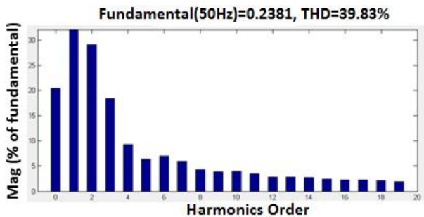
Fig. 14. THD of PCC current for SMS method
