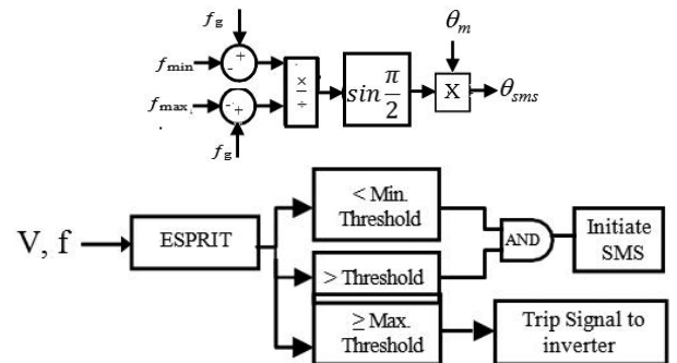
Fig. 2. Proposed hybrid ESPRIT-SMS method
