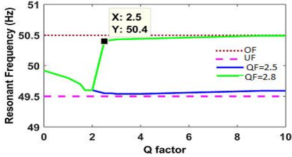
Fig. 4. NDZ of the proposed method
