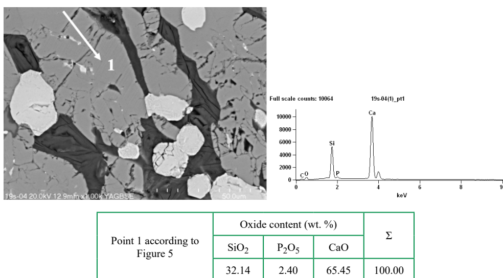
Fig. 5. Dicalcium silicates in aggregate based on open-hearth slag, BSE
