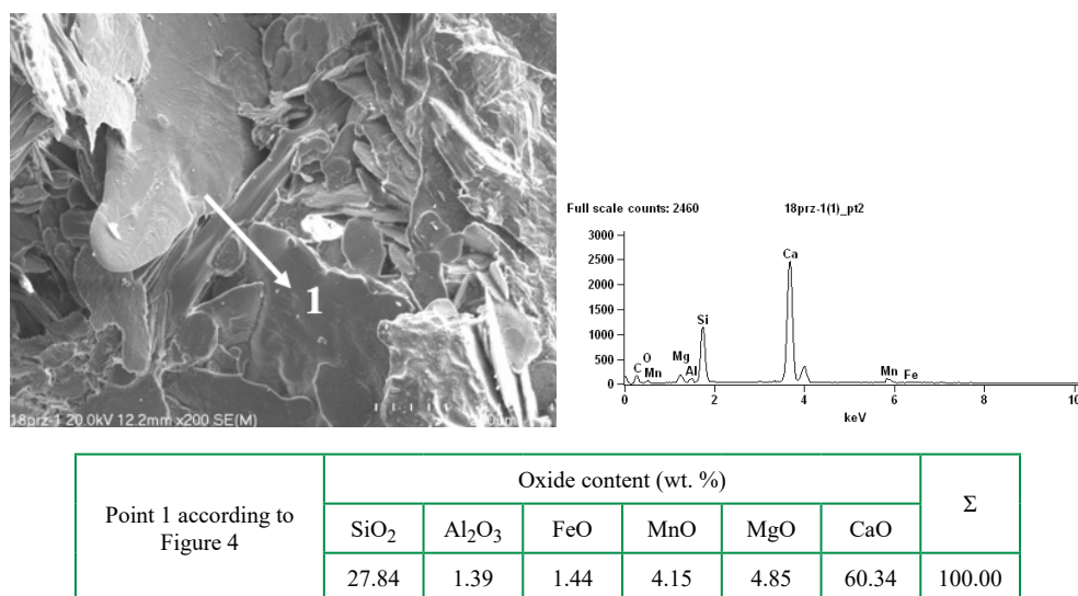
Fig. 4. Dicalcium silicates in aggregate based on open-hearth slag, SEM
