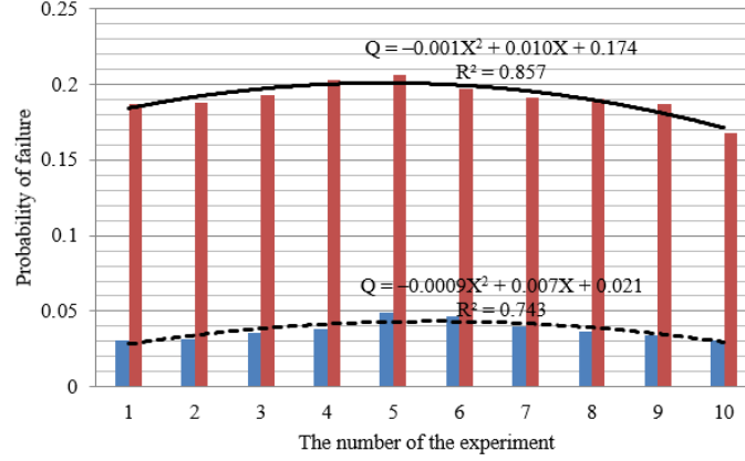
Figure 6: Dependence of the change in the probability of failure of the main equipment on the number of the experiment (simulation model) for the entire population of the studied thermal power plants TPP_1, TPP_2.
