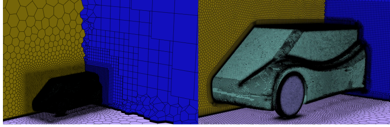
Figure 7: Poly-hexcore mesh around the vehicle.
