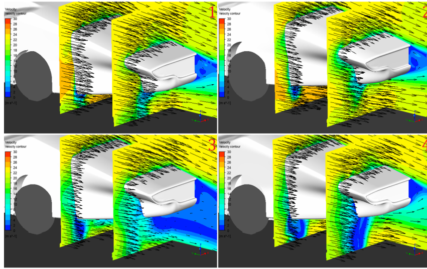
Figure 9: Velocity field towards the rear of the vehicles.
