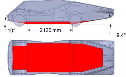
Figure 3: Eagle Two variant 3.
