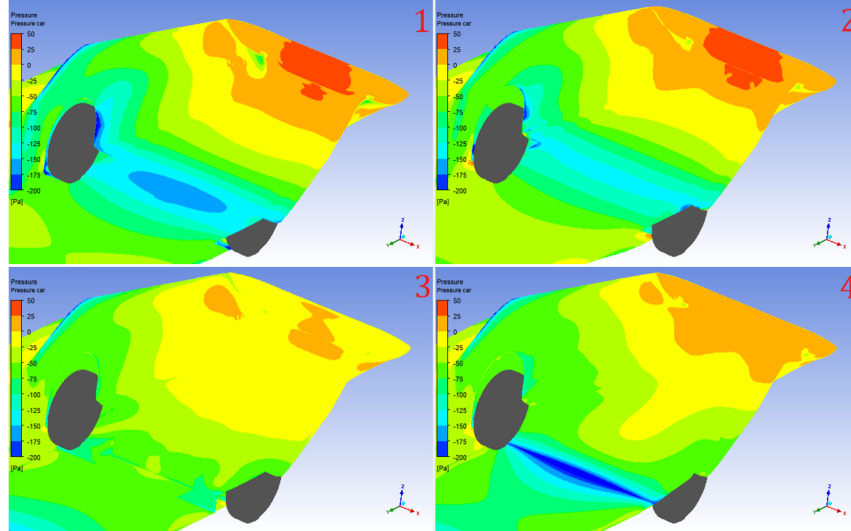
Figure 10: Pressure distribution towards the rear of the vehicles.
