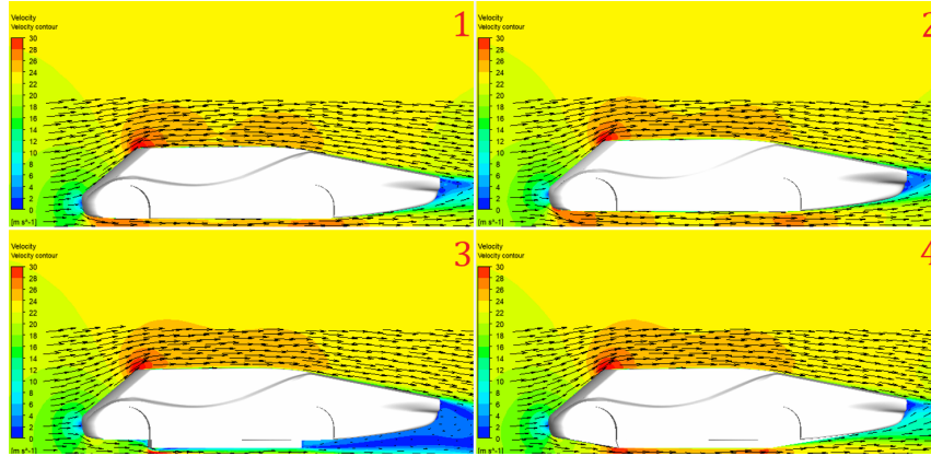
Figure 8: Velocity field at the symmetry plane.
