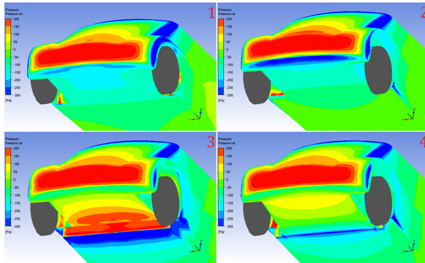
Figure 11: Pressure distribution at the front ends of the vehicles.
