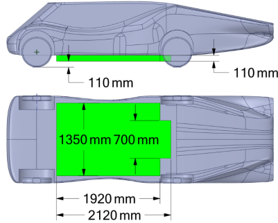
Figure 4: Eagle Two variant 4.
