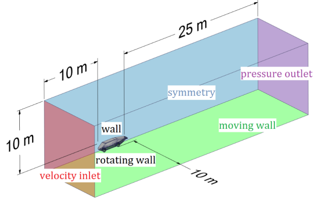
Figure 6: Enclosure around the vehicle.
