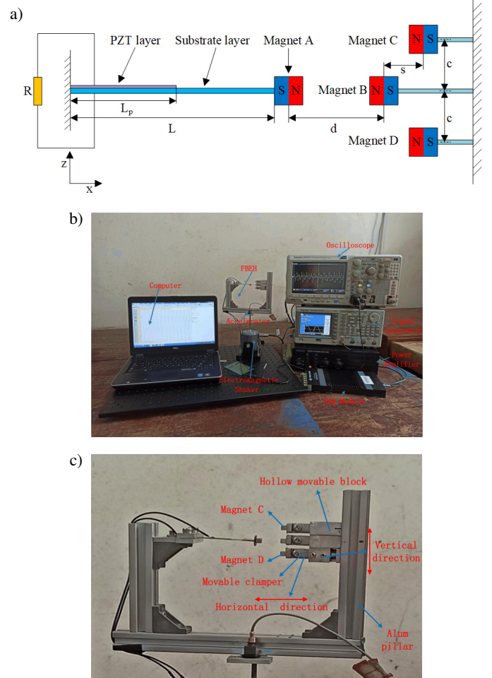
Fig. 1. Proposed FBEH configuration: (a) schematic diagram of FBEH; (b) experimental setup for further research; (c) configuration of magnet C and D for position adjustment
