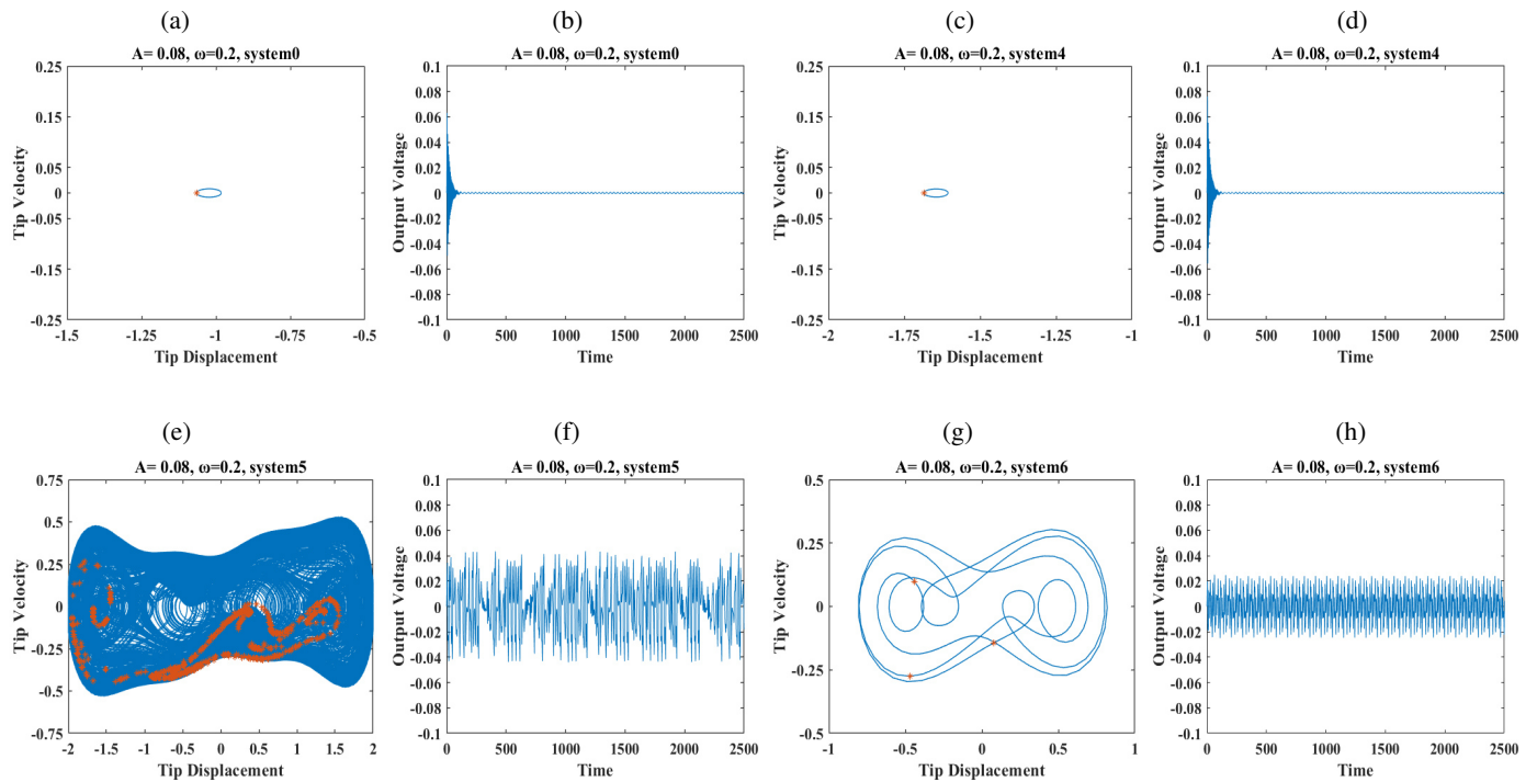
Fig. 12. Phase diagram (blue lines), Poincaré map (red points) and voltage response at \omega = 0.2 and A = 0.08 for (a) and (b) system 0; (c) and (d) system 4; (e) and (f) system 5; (g) and (h) system 6
