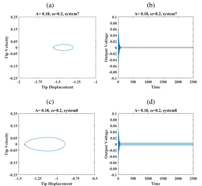
Fig. 17. Phase diagram (blue lines in left column), Poincaré map (red points in left column) and voltage response (right column) at \omega = 0.2 and A = 0.18 for (a) and (b) system 7; (c) and (d) system 8; (e) and (f) system 9
