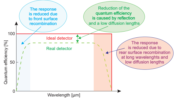
Fig. 7. Quantum efficiency vs. wavelengths for ideal and real detector
