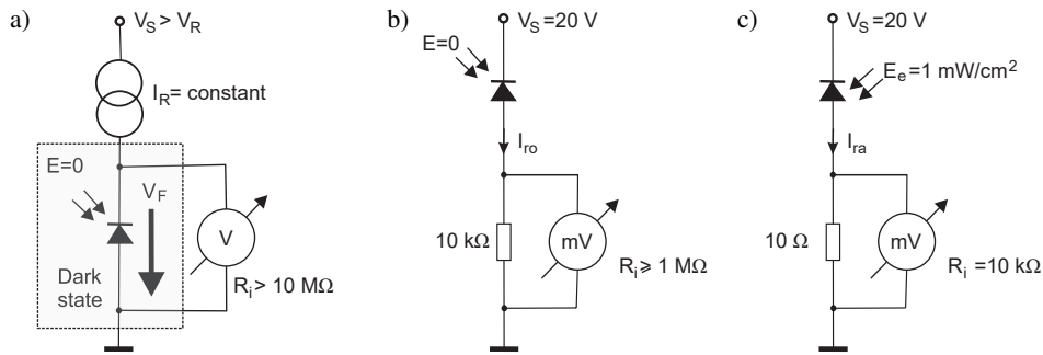
Fig. 15. Equivalent small-signal circuit of a photodiode (where I_d – diode current, I_{Rsh} – shunt resistance current, I_o – output current)
