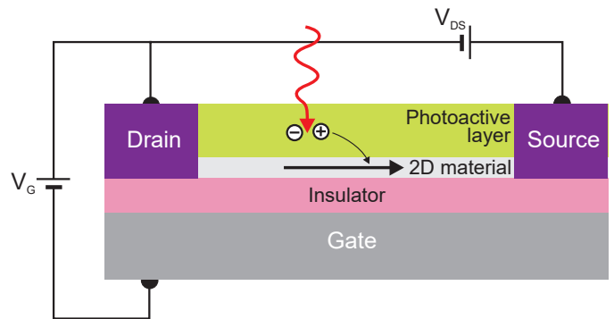
Fig. 3. Operation of hybrid phototransistor
