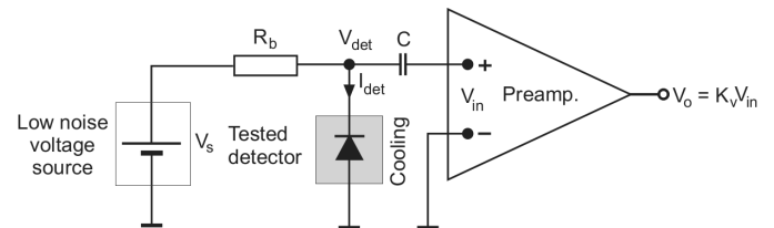
Fig. 24. Detector noise measurement circuit with voltage amplifier
