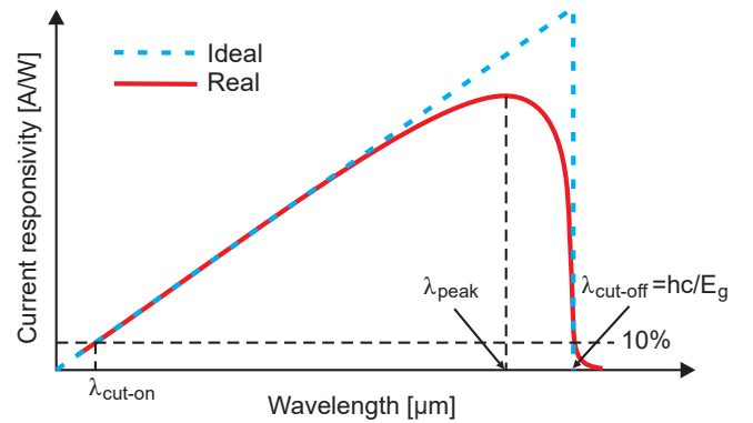
Fig. 8. Relative current responsivity of ideal and real photodiodes
