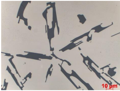
Fig. 8. The morphology of eutectic silicon in the central part of casting, 1000x magnification; sand mould
