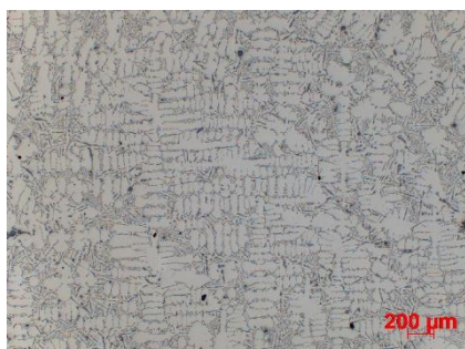
Fig. 4. The dispersion of dendritic structure in the central part of casting, 50x magnification: ablation mould
