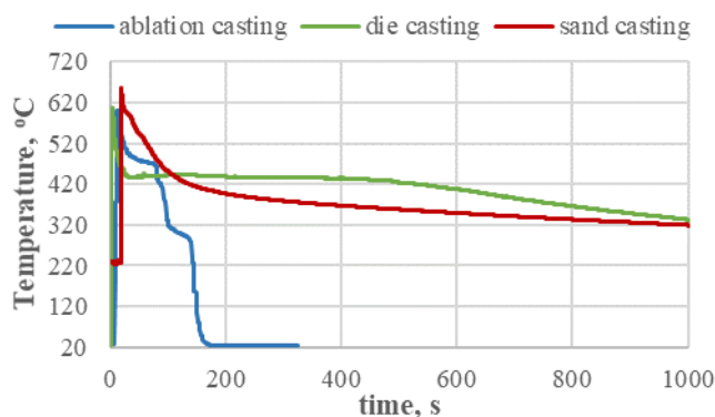
Fig. 3. Cooling curves recorded in moulds during melting
