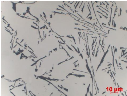
Fig. 9. The morphology of eutectic silicon in the central part of the casting, 1000x magnification; metal mould
