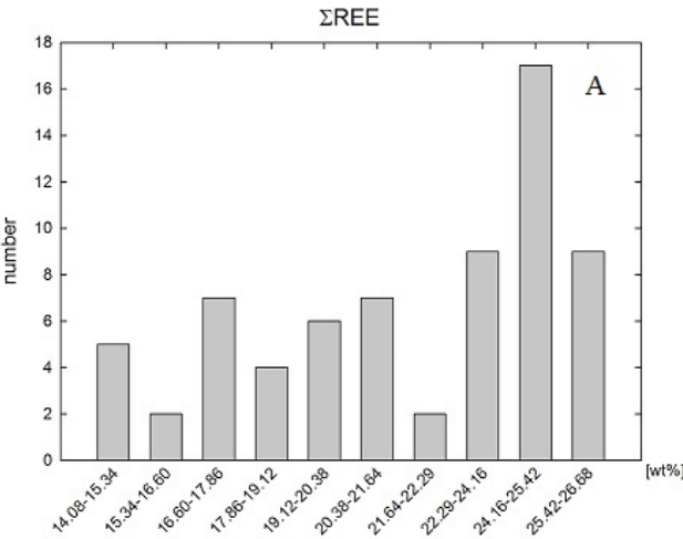
Fig. 13A. Histogram of REE content in allanites
