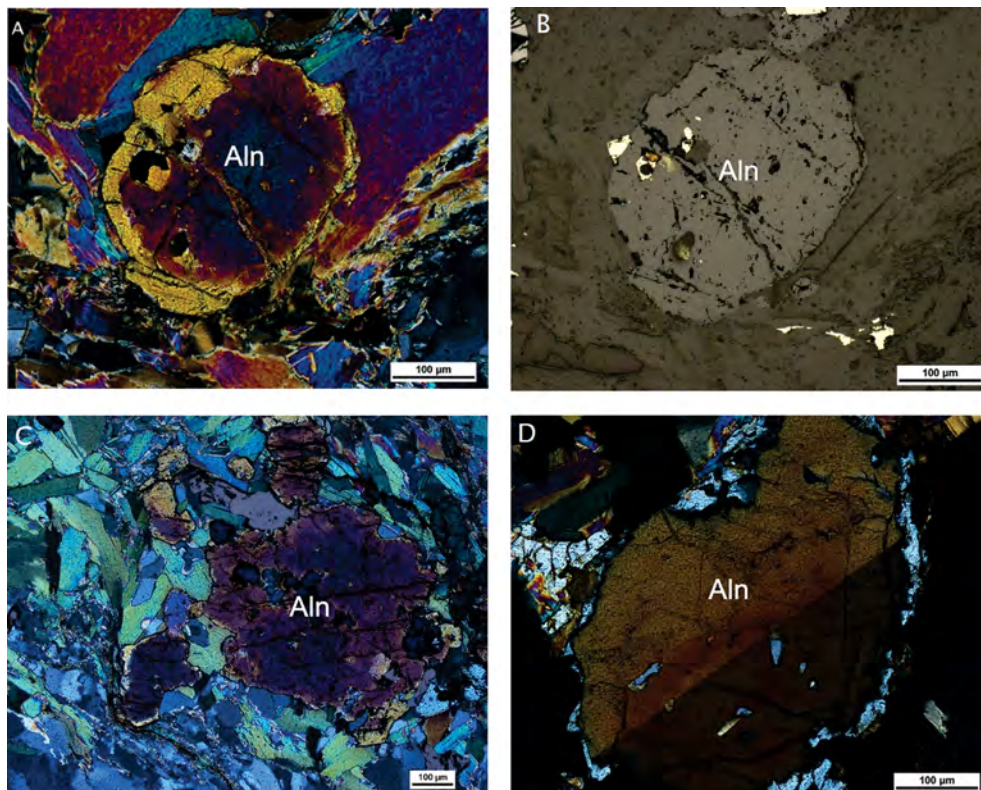
Fig. 5. Microphotographs of ore minerals from Sin Quyen deposit in transmitted (TL) and reflected light (RL) A – Allanite crystal in pyroxene matrix (TL), B – Allanite grain with sulphide inclusions (RL), C – altered allanite in pyroxene matrix (TL), D – allanite twins (TL)
