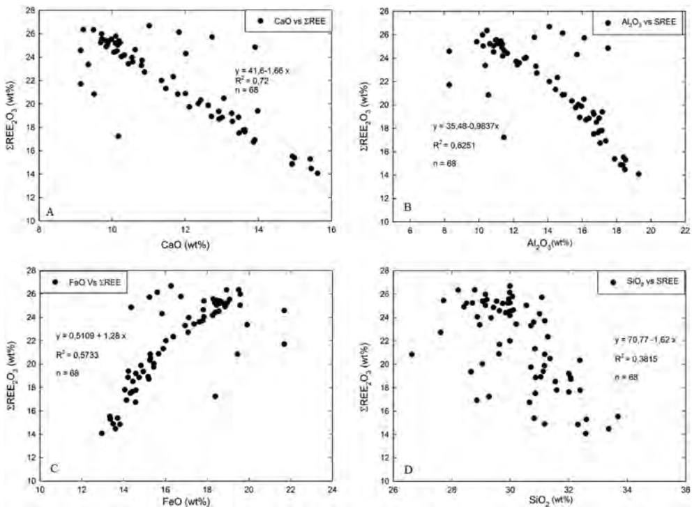
Fig. 8. Correlation between \Sigma\text{REE} and \text{CaO} , \text{Al}_2\text{O}_3 , \text{FeO} , \text{SiO}_2 in allanite
