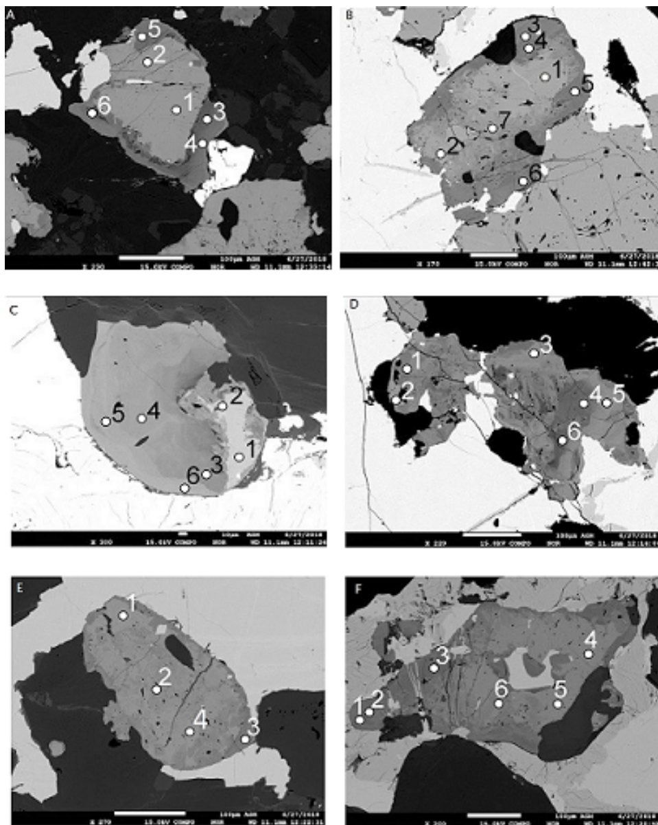
Fig. 6. Selected BSE-WDS (A–F) images of analyzed allanite grains. Gray shadows show changing in chemical composition. Numbers on the pictures show positions of WDS measurements, sample N4 A – black are silicate, white-sulphides, B – white are sulphides, C – black are silicate, white-sulphides, D – black are silicate, white-sulphides, E – black are silicate, white-sulphides, F – black are silicate, white-sulphides
