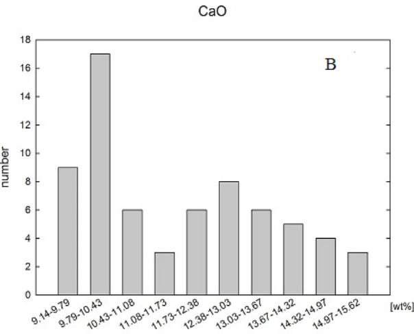
Fig. 13B. Histogram of CaO content in allanites
