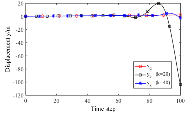
Fig. 15. Tracking curves of y
