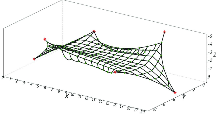
Fig. 14. Hexagonal cable net after removal of 4 elements
