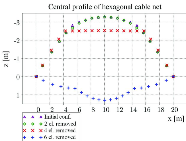
Fig. 18. Central profile of hexagonal cable net in different stages
