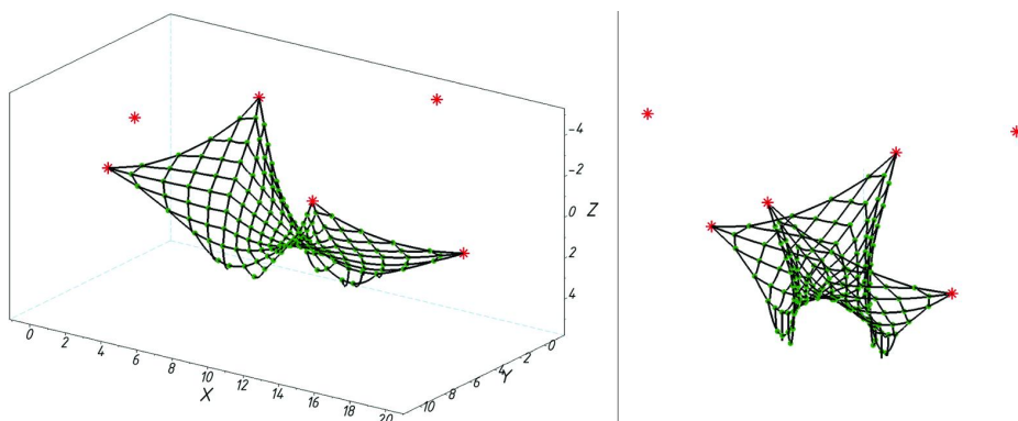
Fig. 16. Hexagonal cable net after removal of 6 elements
