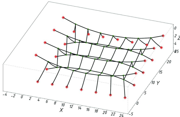
Fig. 7. Sawtooth roof with self-weight and unstretched lengths taken from step 2 (step 4)
