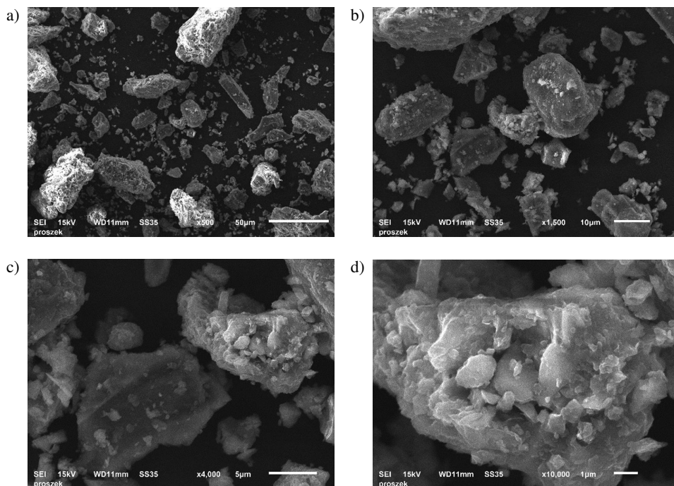
Fig. 2. The image of rock dust created using scanning electron microscopy SEM Joel JSM-6610 (Joel, Tokyo, Japan) a) 500 \times , b) 1500 \times , c) 4000 \times , d) 10000 \times
