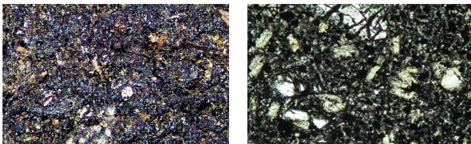
Fig. 1. Diabase structure
