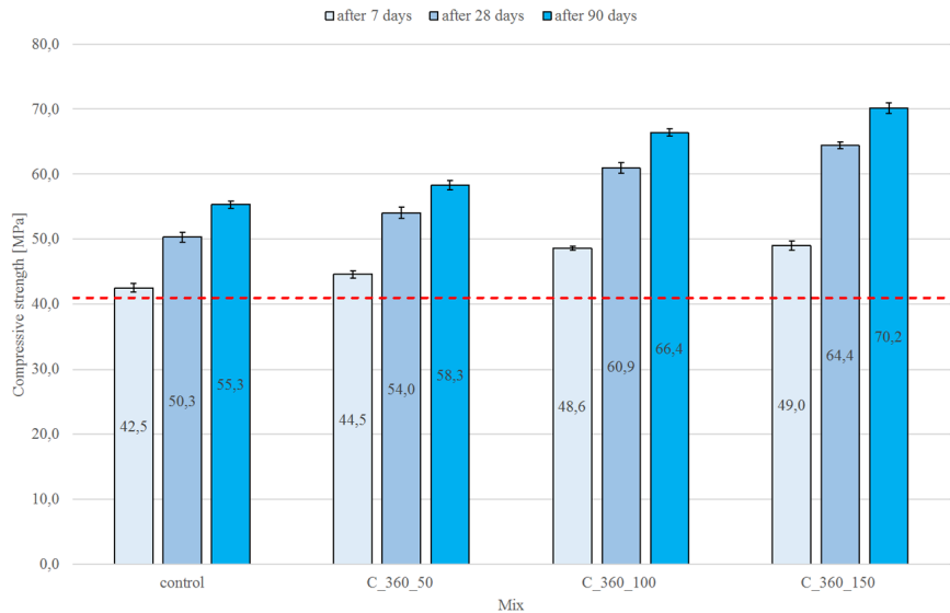
Fig. 4. The influence of diabase dust, as a filler, on compressive strength
