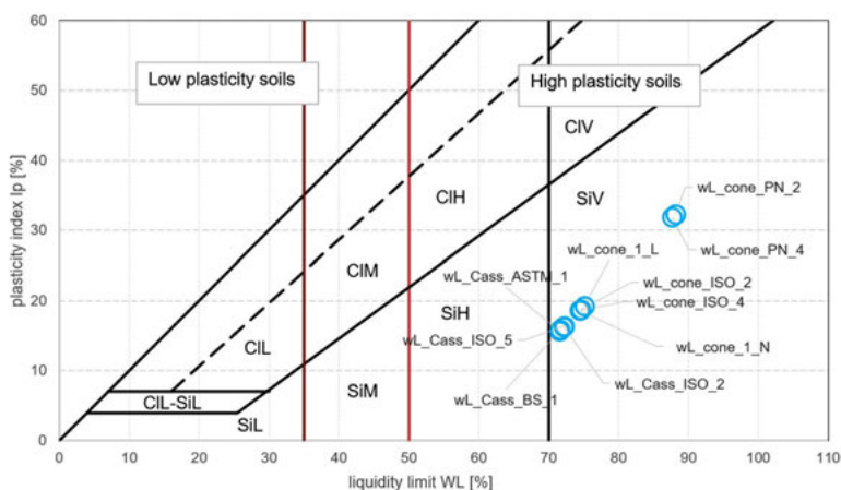
Fig. 12. The result of plasticity on the Cassagrande plasticity chart [41] for soil No. 2 ( LOI_T = 48.71\% )
