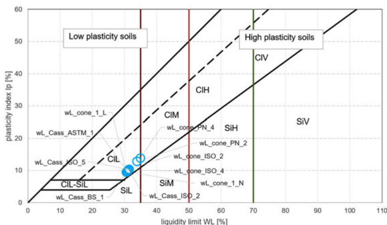
Fig. 11. The result of plasticity on the Cassagrande plasticity chart [41] for soil No. 1 ( LOI_T = 7.71\% )
