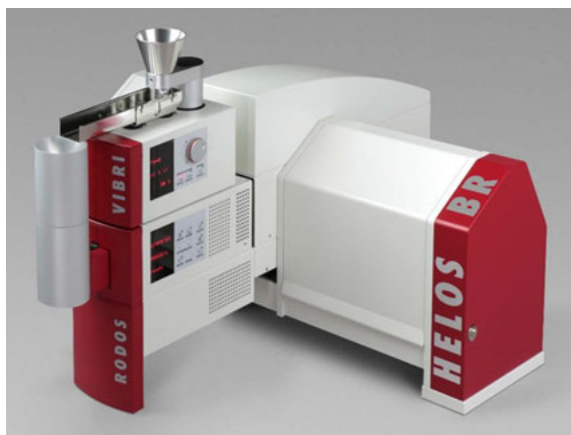
Fig. 2. The set for dry measurements: HELOS diffractometer, RODOS dispersant, VIBRI feeder [37]
