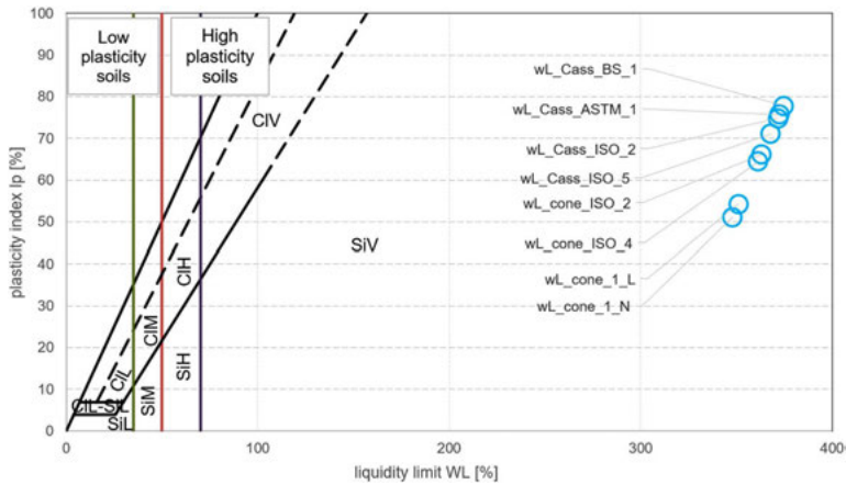
Fig. 13. The result of plasticity on the Cassagrande plasticity chart [41] for soil No. 3 ( LOI_T = 70.84\% )
