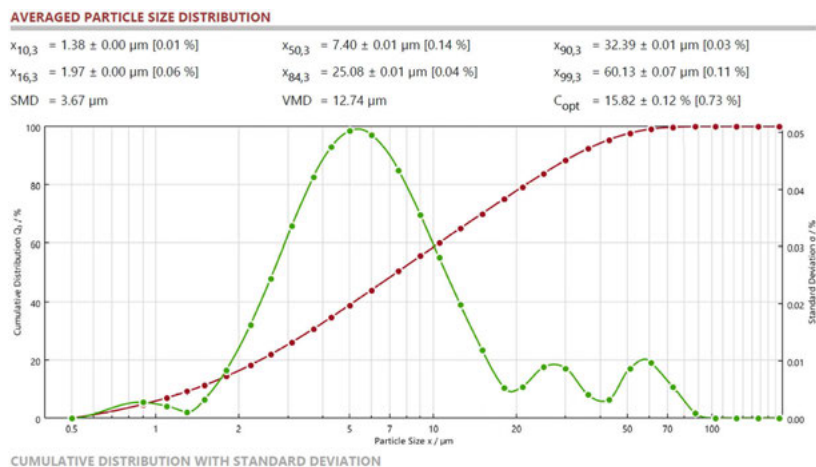
Fig. 5. The average particle size distribution by Laser Diffractometer for soil No. 1 ( \text{LOI}_T = 7.71\% )
