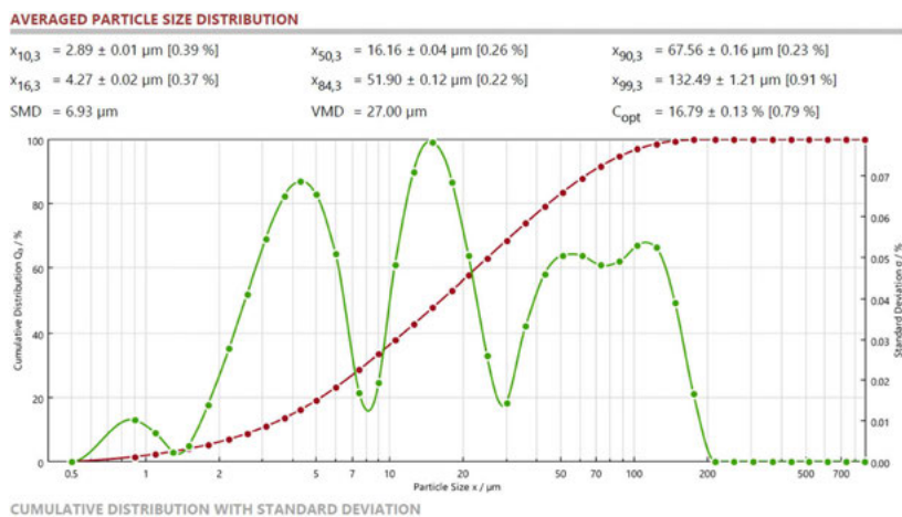
Fig. 6. The average particle size distribution by Laser Diffractometer for soil No. 2 ( \text{LOI}_T = 48.71\% )
