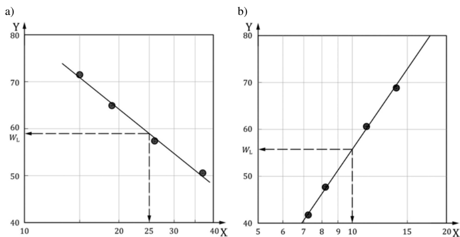
Fig. 3. The example of a the liquid limit test result based to the rules of the standard [35] from: a) the Casagrande cup test and b) the fall cone test
