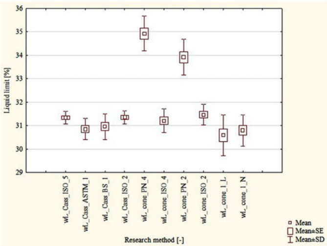
Fig. 8. The mean values of liquidity limits into account Standard Error (SE) and Standard Deviation (SD) of soils No. 1 ( LOI_T = 7.71\% ), depending on the determination method
