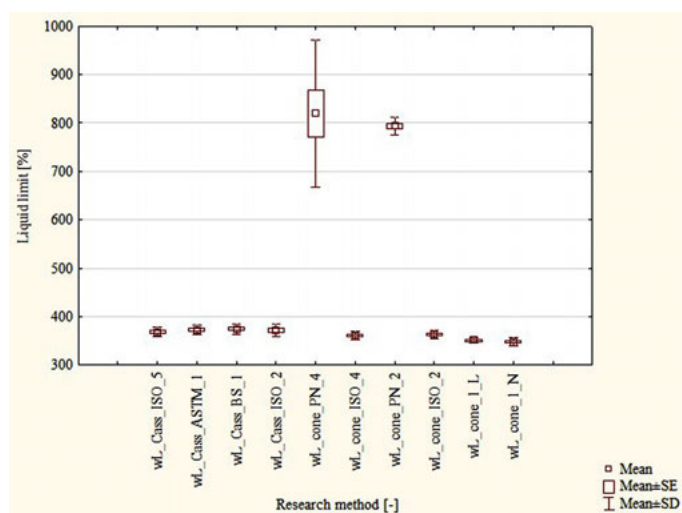
Fig. 10. The mean values of liquidity limits into account Standard Error (SE) and Standard Deviation (SD) of soils No. 3 ( LOI_T = 70.84\% ) depending on the determination method
