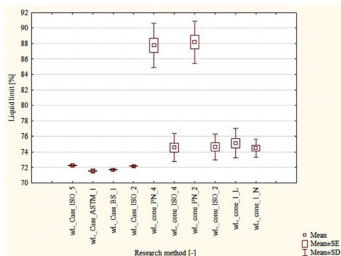
Fig. 9. The mean values of liquidity limits into account Standard Error (SE) and Standard Deviation (SD) of soils No. 2 ( LOI_T = 48.71\% ) depending on the determination method
