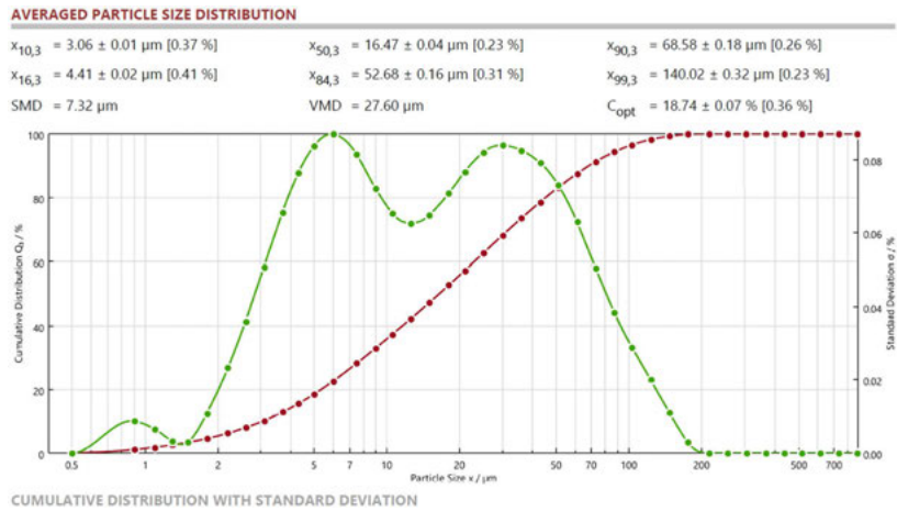
Fig. 7. The average particle size distribution by Laser Diffractometer for soil No. 3 ( LOI_T = 70.84\% )
