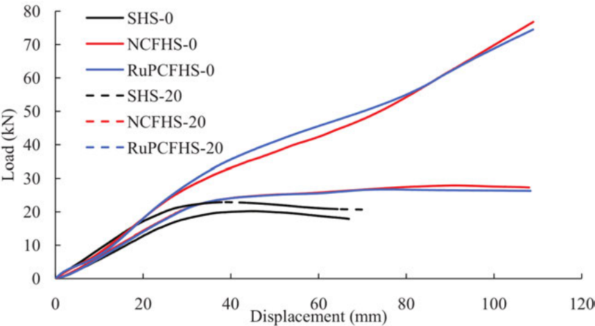
Fig. 5. Load-deflection curves of columns under lateral load
