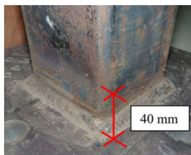
(b) Deformation of SHS-20
