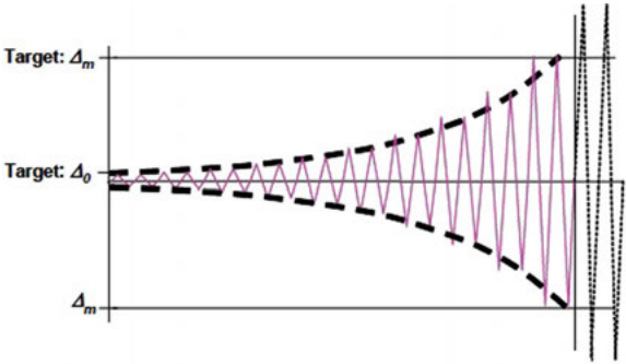
Fig. 4. FEMA 461 cyclic loading history [16]
