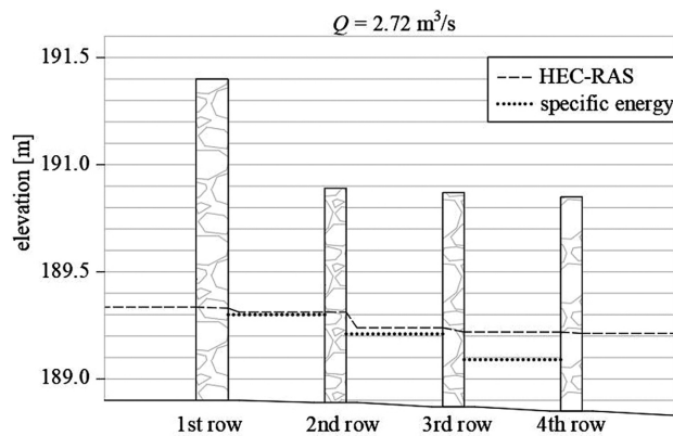
Fig. 11. Comparison of calculated water table elevations for a discharge of Q = 2.72 m 3 /s
