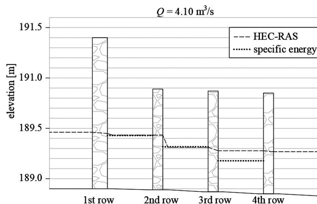
Fig. 12. Comparison of calculated water table elevations for a discharge of Q = 4.10 m 3 /s
