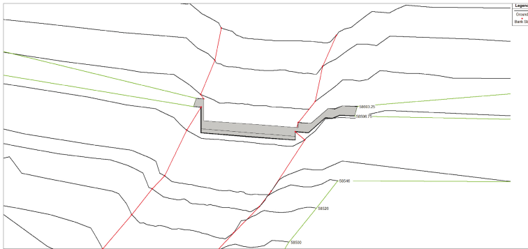
Fig. 7. Computational model of existing river bed generated in HEC–RAS
