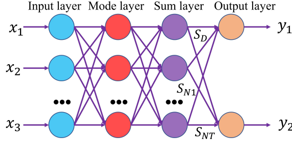
Fig. 4. GRNN structure.
