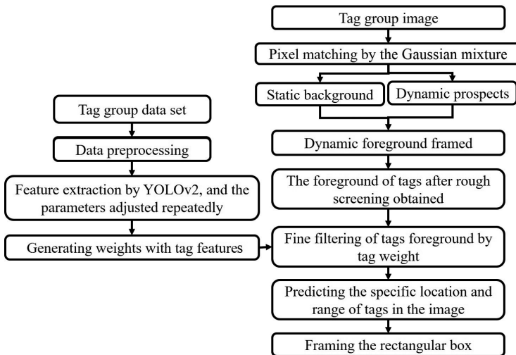
Fig. 8. Flow chart of tags group recognition algorithm YOLOv2 improved with the Gaussian filter.
