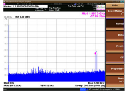
d) mode without digital resampling ( f_{s2} = 2 GSPS)
