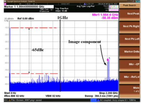
b) mode without digital resampling ( f_{s2} = 2 GSPS)
