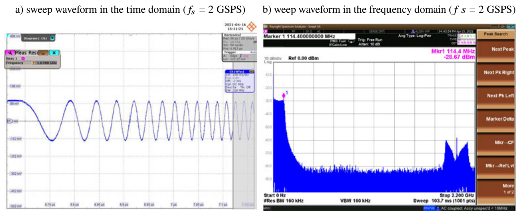
Fig. 10. Test results for the sweep waveform.
