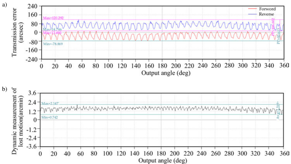
Fig. 1. Process of obtaining the dynamic measurement curve of the lost motion: a) Forward and reverse transmission errors; b) Dynamic measurement curve of the lost motion.
