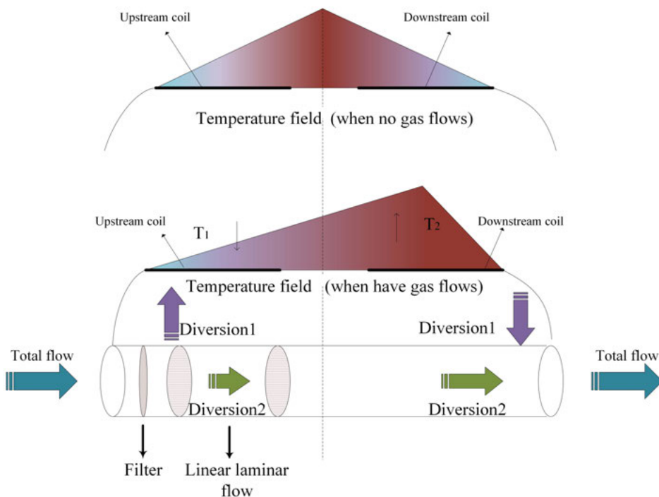
Fig. 2. Measuring principle of the digital thermal flowmeter.
