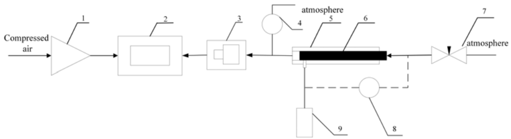
Fig. 3. Diagram of the differential pressure compensation principle for ventilation rate measurement based on a digital thermal flowmeter: 1. gas pressure regulator; 2. negative pressure generator; 3. tobacco special standard constant flow hole; 4. differential pressure sensor 1; 5. special fixture; 6. tobacco special ventilation rate standard rod; 7. needle valve; 8. differential pressure sensor 2; 9. digital thermal flow sensor.
