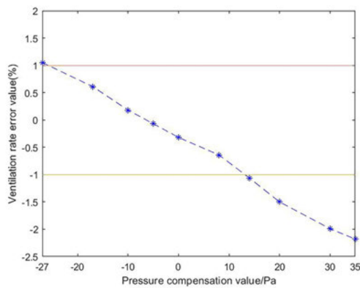
Fig. 8. Relationship between the experimental and verification values for the standard bar with a 71.95% ventilation rate.
