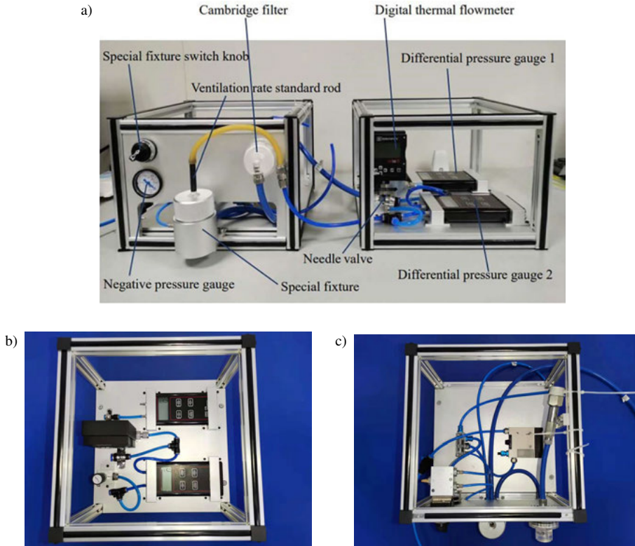
Fig. 5. Overall experimental installation set-up a) with the top views of the left b) and right boxes c).
