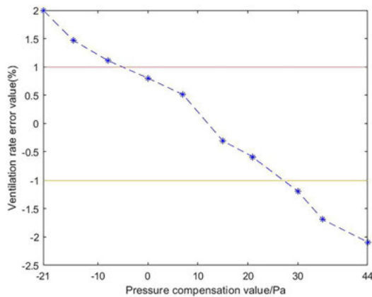
Fig. 7. Relationship between the experimental and verification values for the standard bar with a 58.83% ventilation rate.
