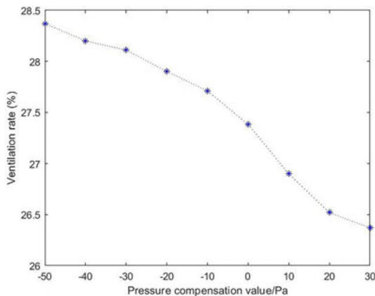
Fig. 4. Ventilation rate curve under different pressure differences.
