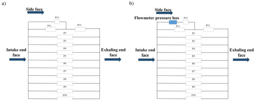
Fig. 1. Ventilation rate standard rod pressure drop model: a) no flowmeter introduced; b) flowmeter introduced.
