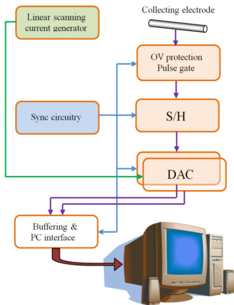
Fig.4. Configuration of data collecting hardware
