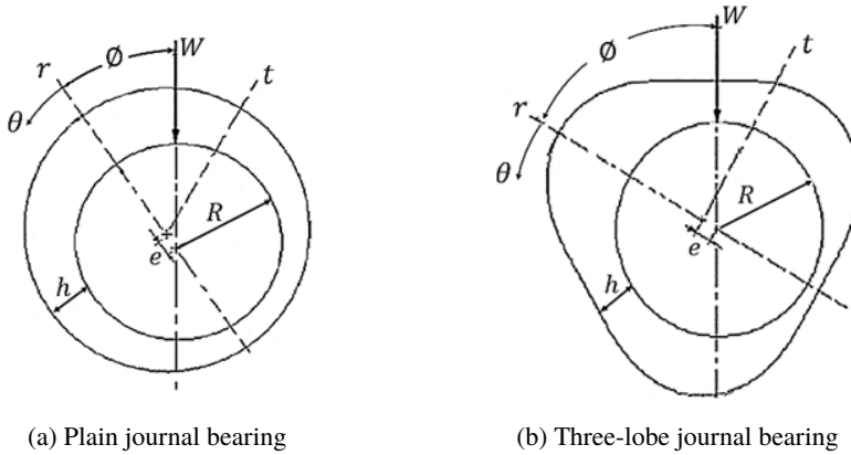
Fig. 1. Geometry of cylindrical and three lobe journal bearings [9]
