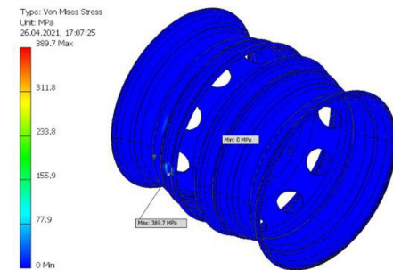
Fig. 20. The von Mises stress distribution in the assembly of the modelled rims for the case of transport of pallets with paving stones during driving on the dirt road when case only one tire of the one twin wheel of the rear axle were in contact with the road
