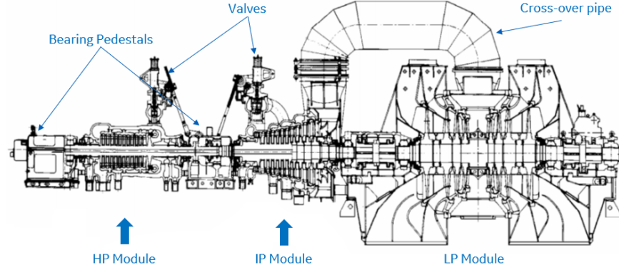
Figure 1: Longitudinal section of a 13K215 turbine.
