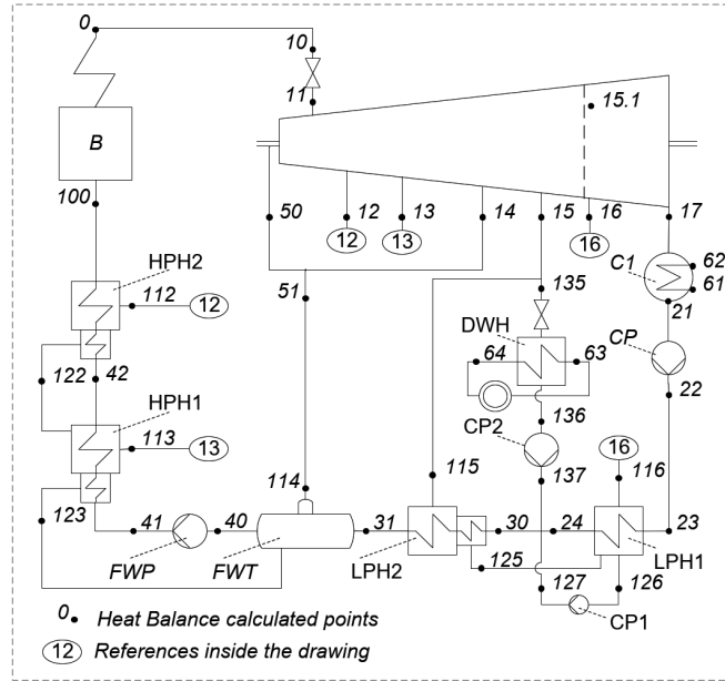
Figure 1: Tested thermal cycle scheme – CHP plant (A).
