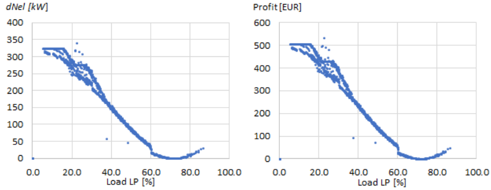
Figure 23: Optimization profit – cooling tower flow limitation actives.
