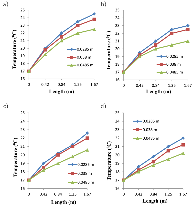
Figure 3: Air temperature variations along the pipes of different diameters at a velocity of (a) 2 m/s, (b) 3.5 m/s, (c) 5 m/s, (d) 6.5 m/s.
