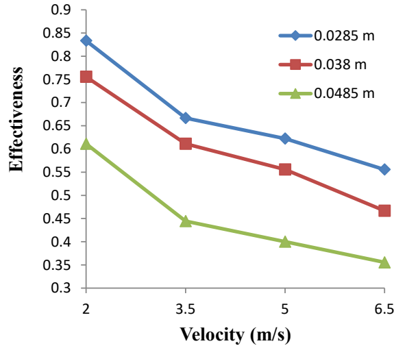
Figure 4: Effectiveness of the EAHE for all the sets of induced air velocities.
