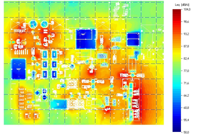
Fig. 3. Map of the industrial plant situation after acoustic treatment.
